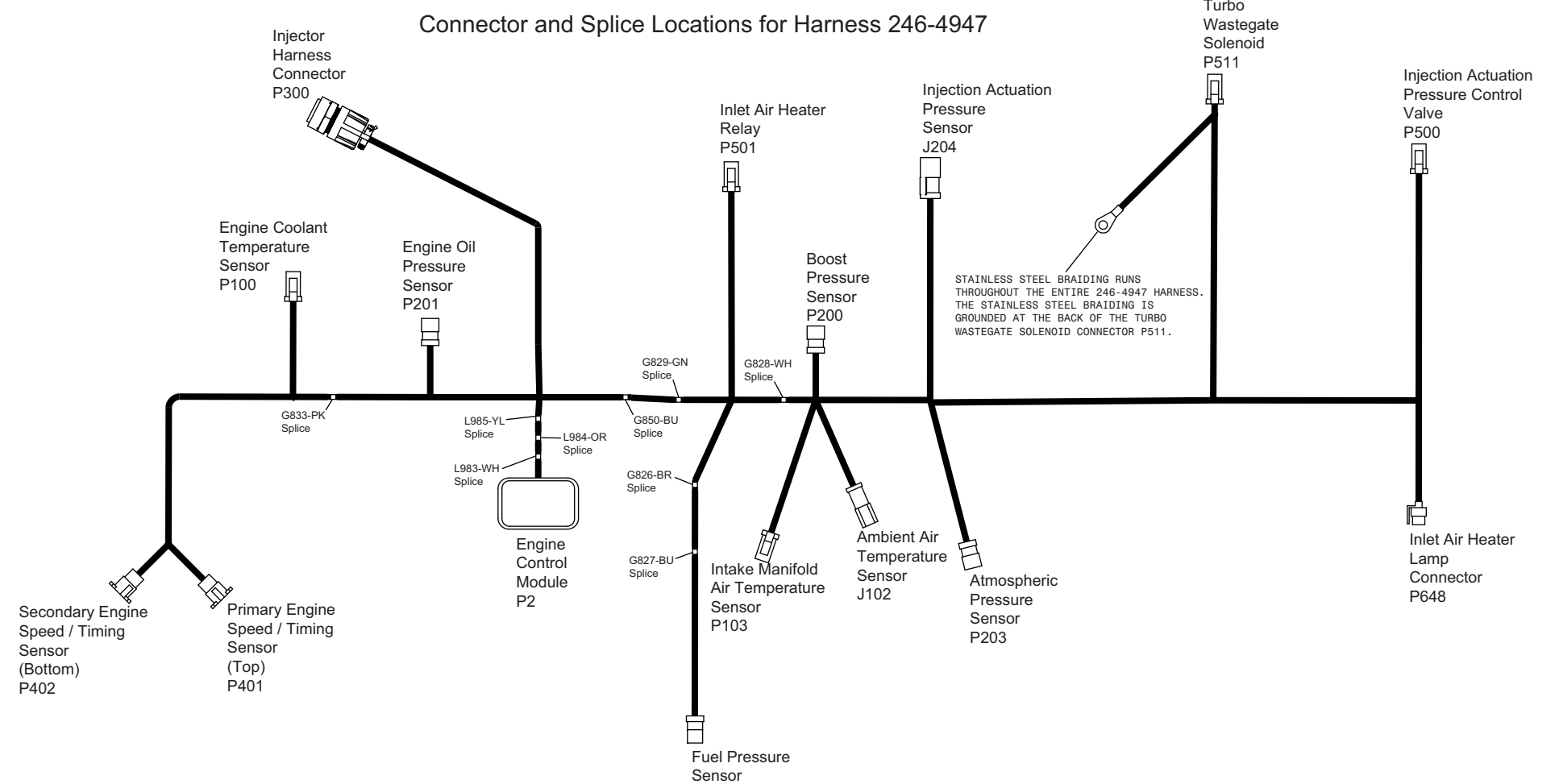
Connector and Splice Locations for Harness 246-4947
