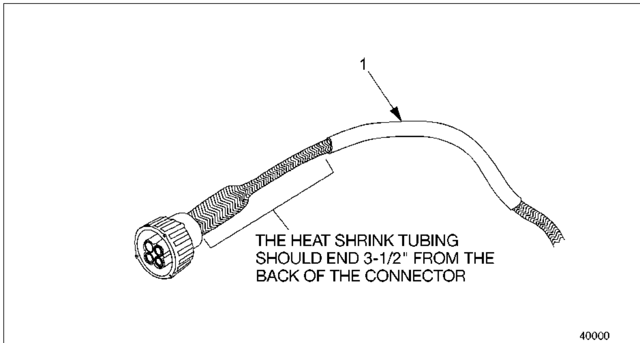
Figure 1. Location of Heat Shrink Tubing
