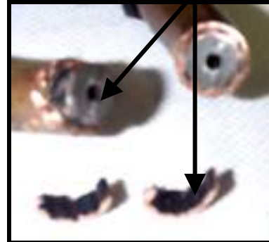
Fig. 69 OVERHEATED & CARBONED FROM LEAKING C-E RING
