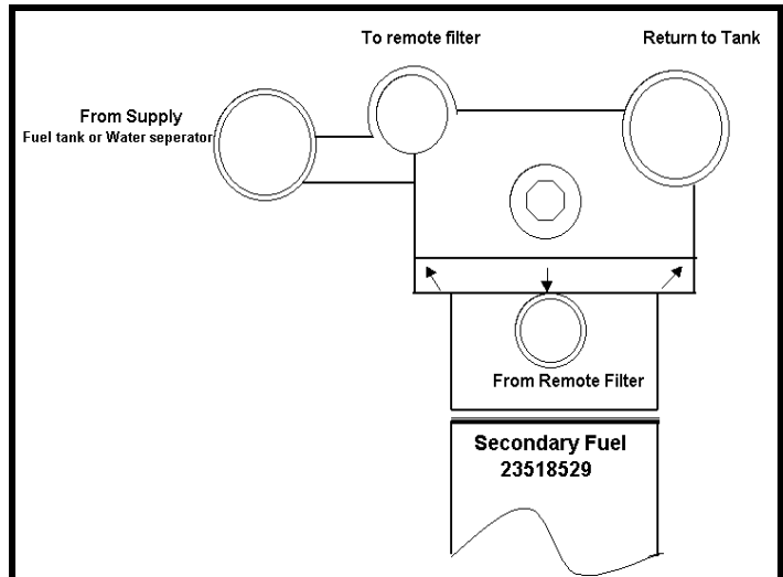
Fig. 105 C&I Fuel Junction Block Off-engine Fuel Line Connection Identification
