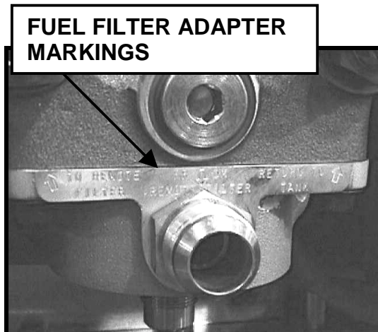
Fig. 105 C&I Fuel Junction Block Off-engine Fuel Line Connection Identification
