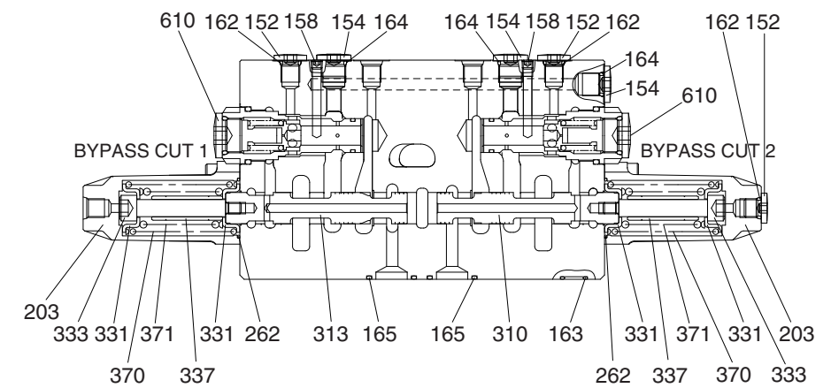
SECTION H-H
