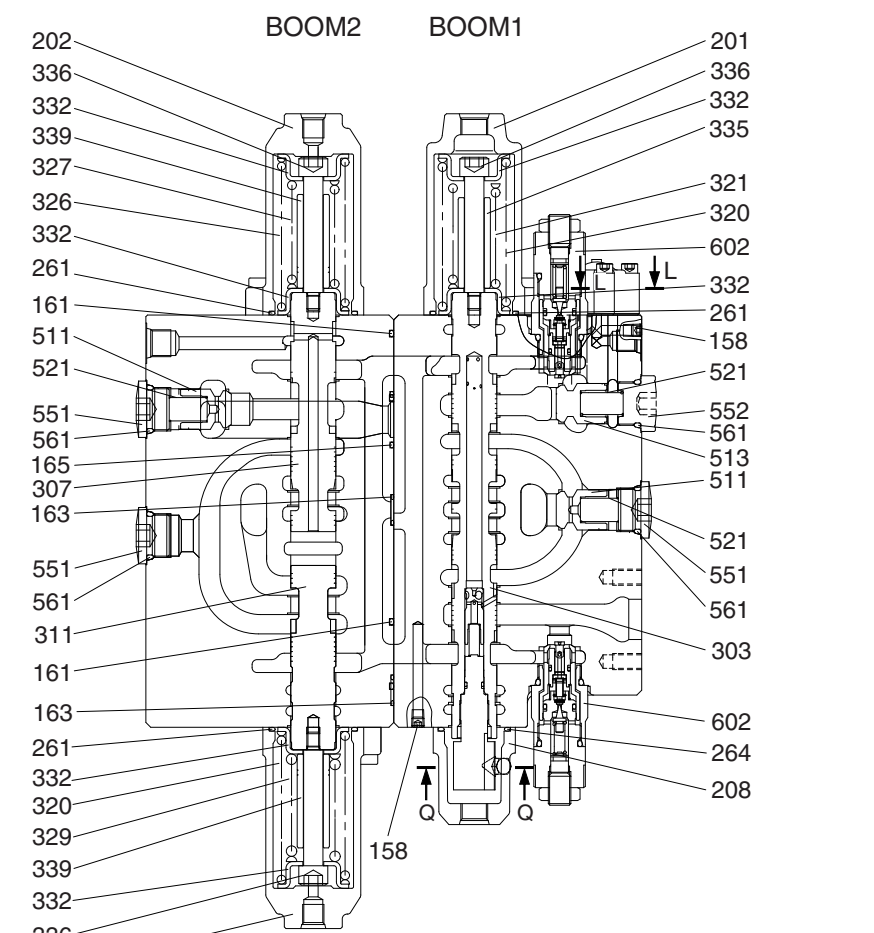
SECTION E-E
