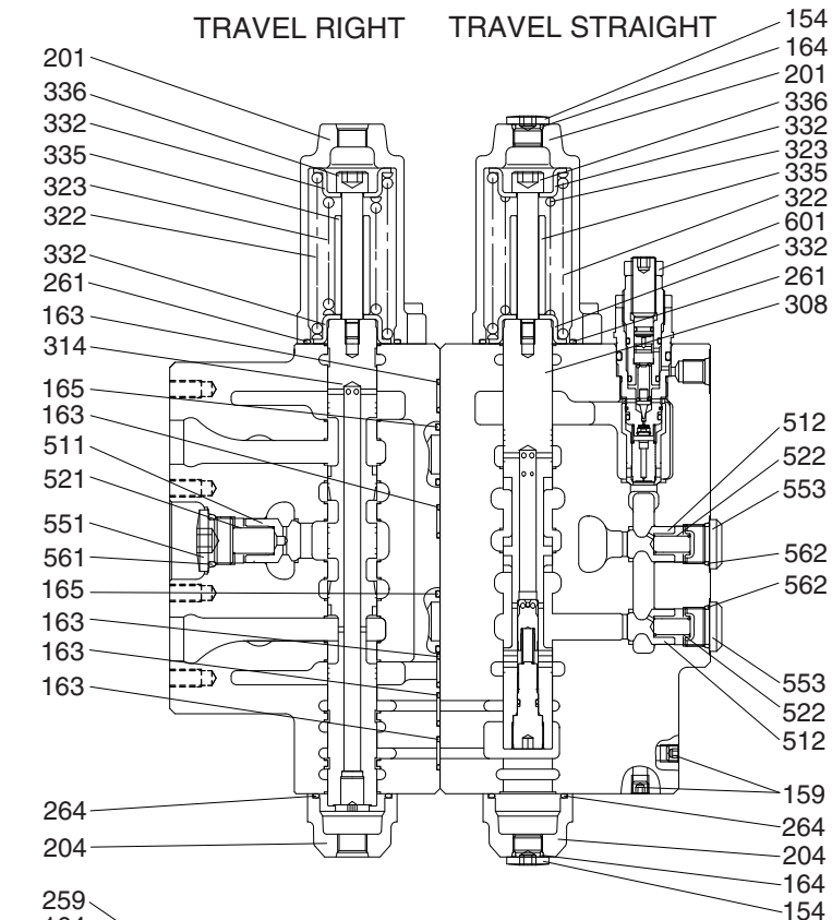
SECTION C-C
