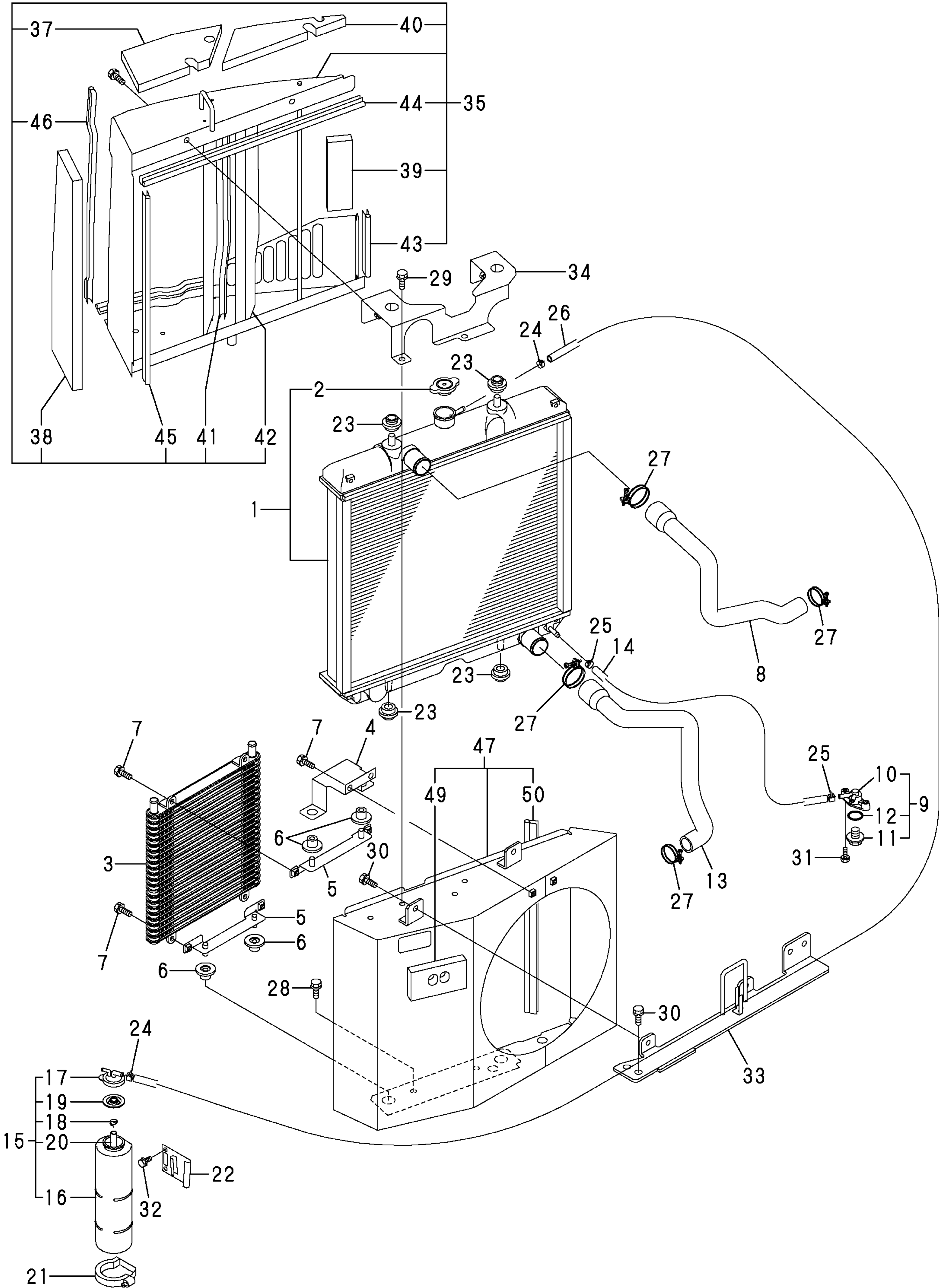
Fig. 5 RADIATOR & MOUNT
