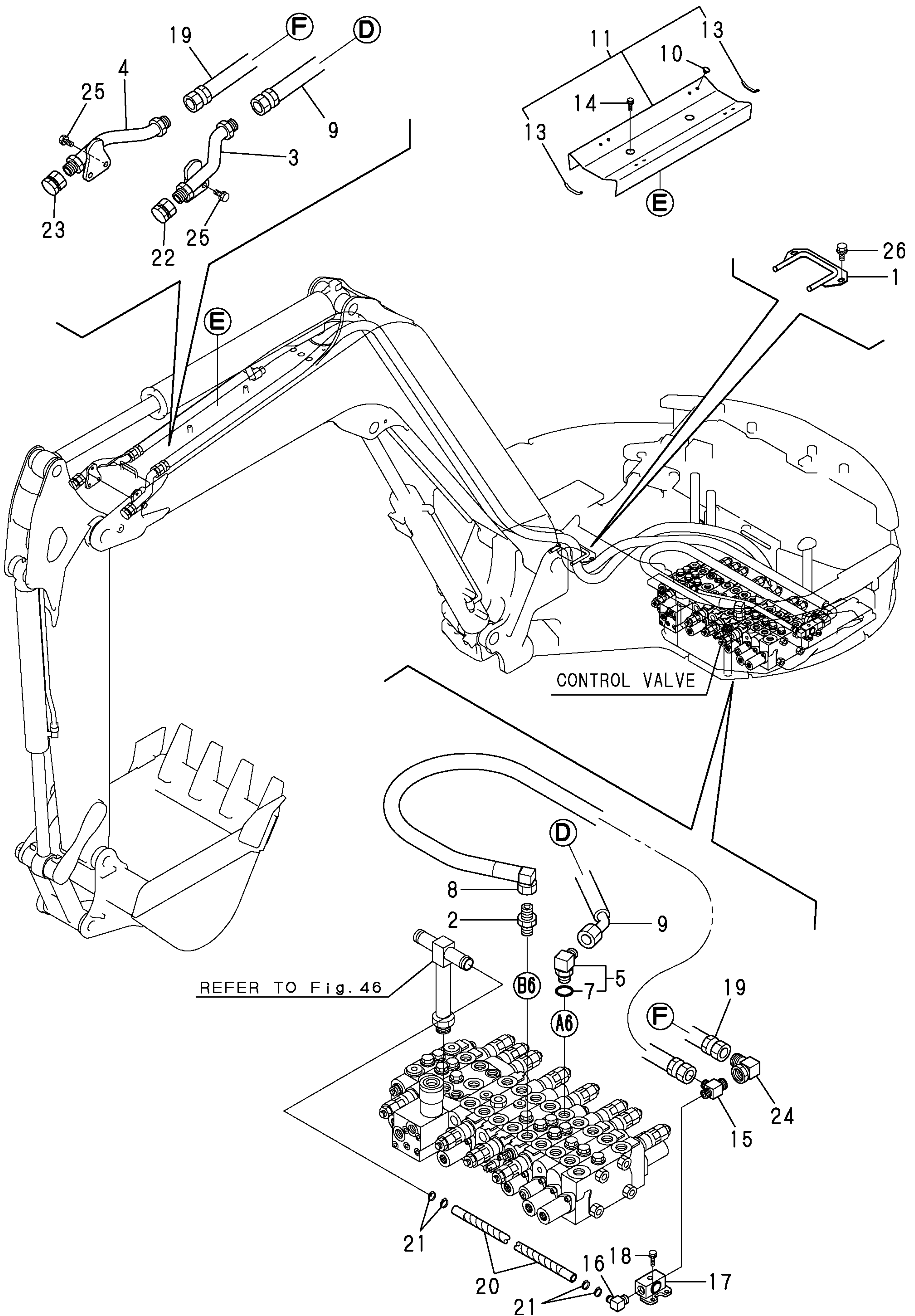
Fig. 49 HYD. OIL PIPING (P. T. O.)
