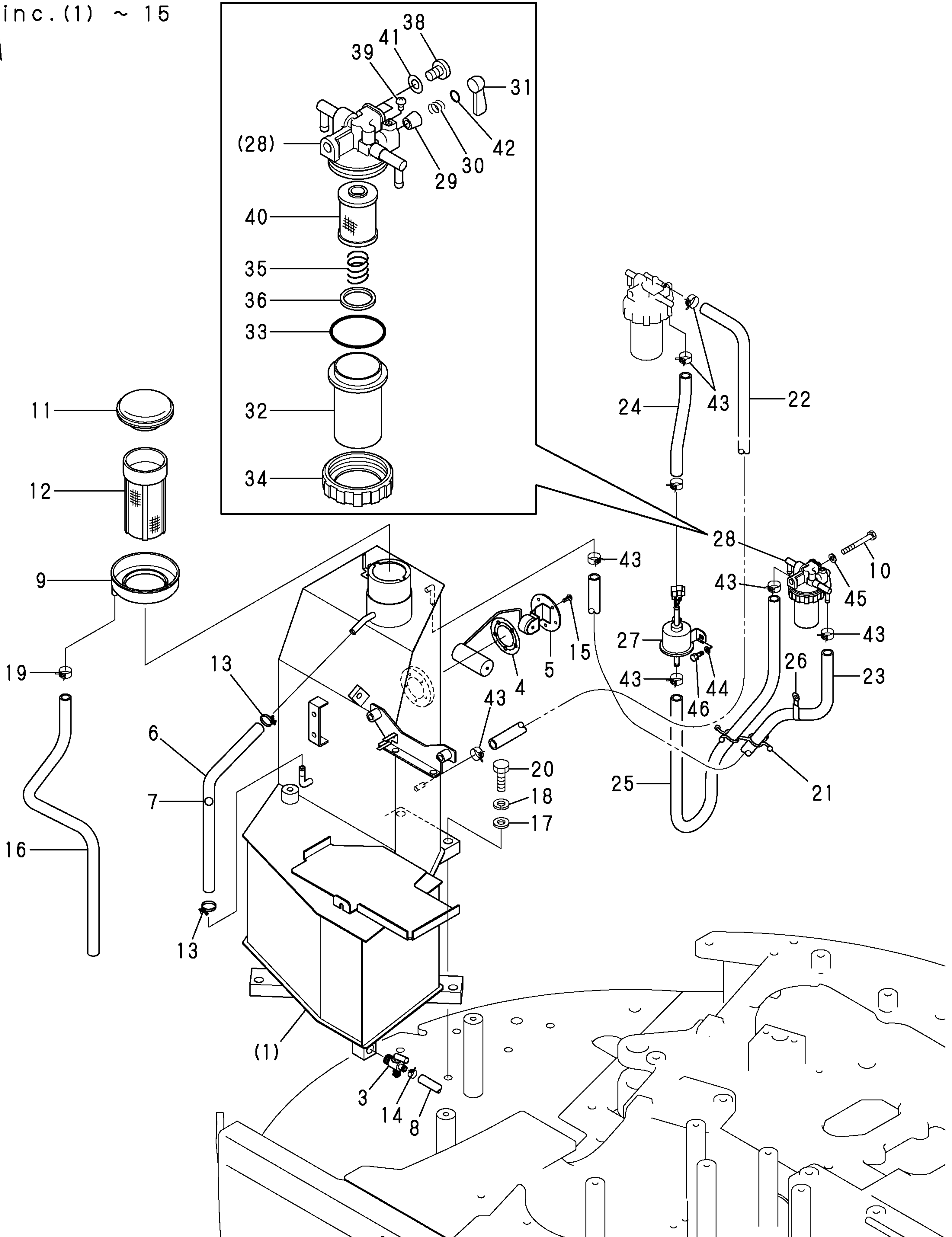
Fig. 6 FUEL TANK & FUEL PIPE
