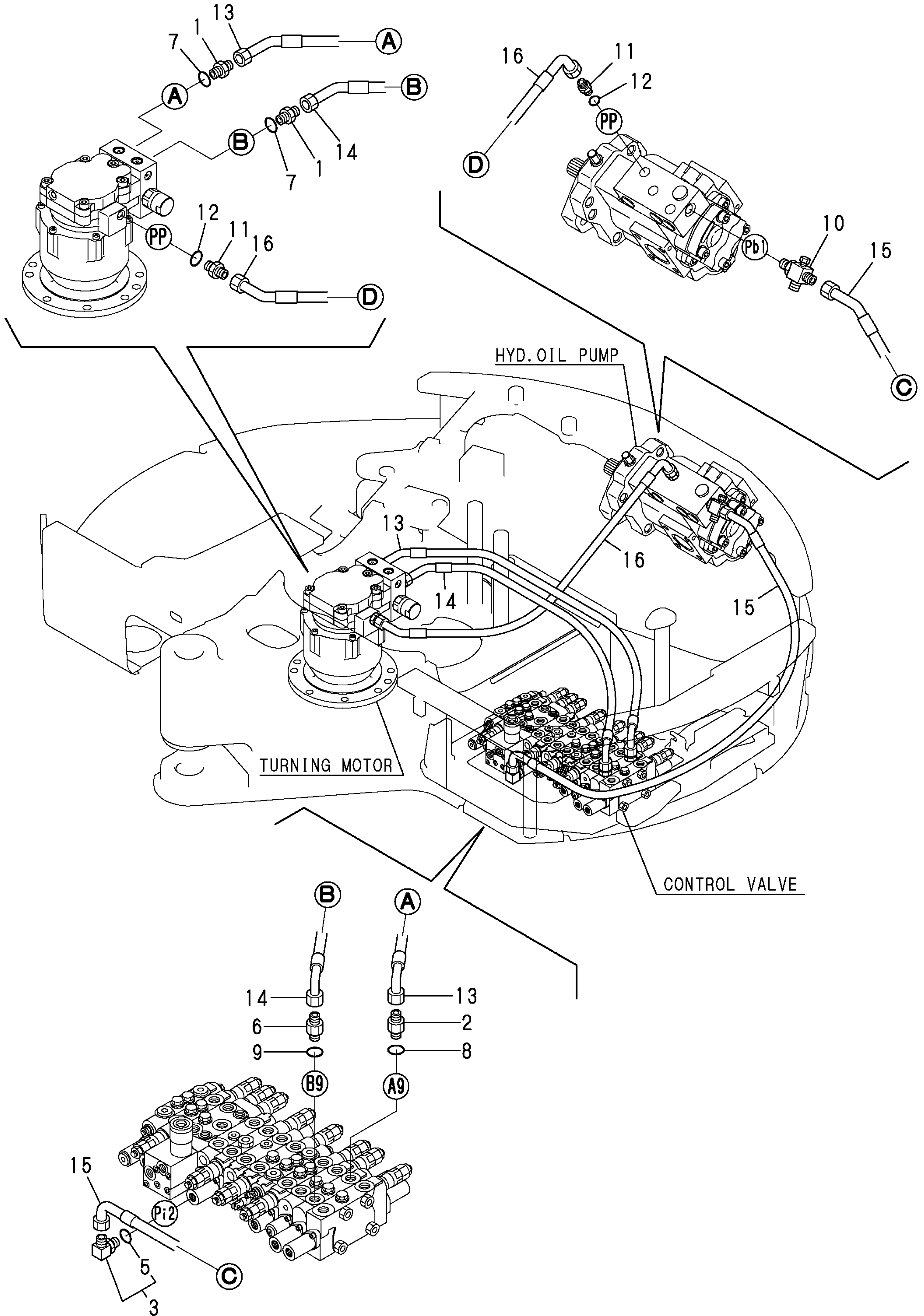
Fig. 44 HYD. OIL PIPING (PUMP-V. -MOTOR)
