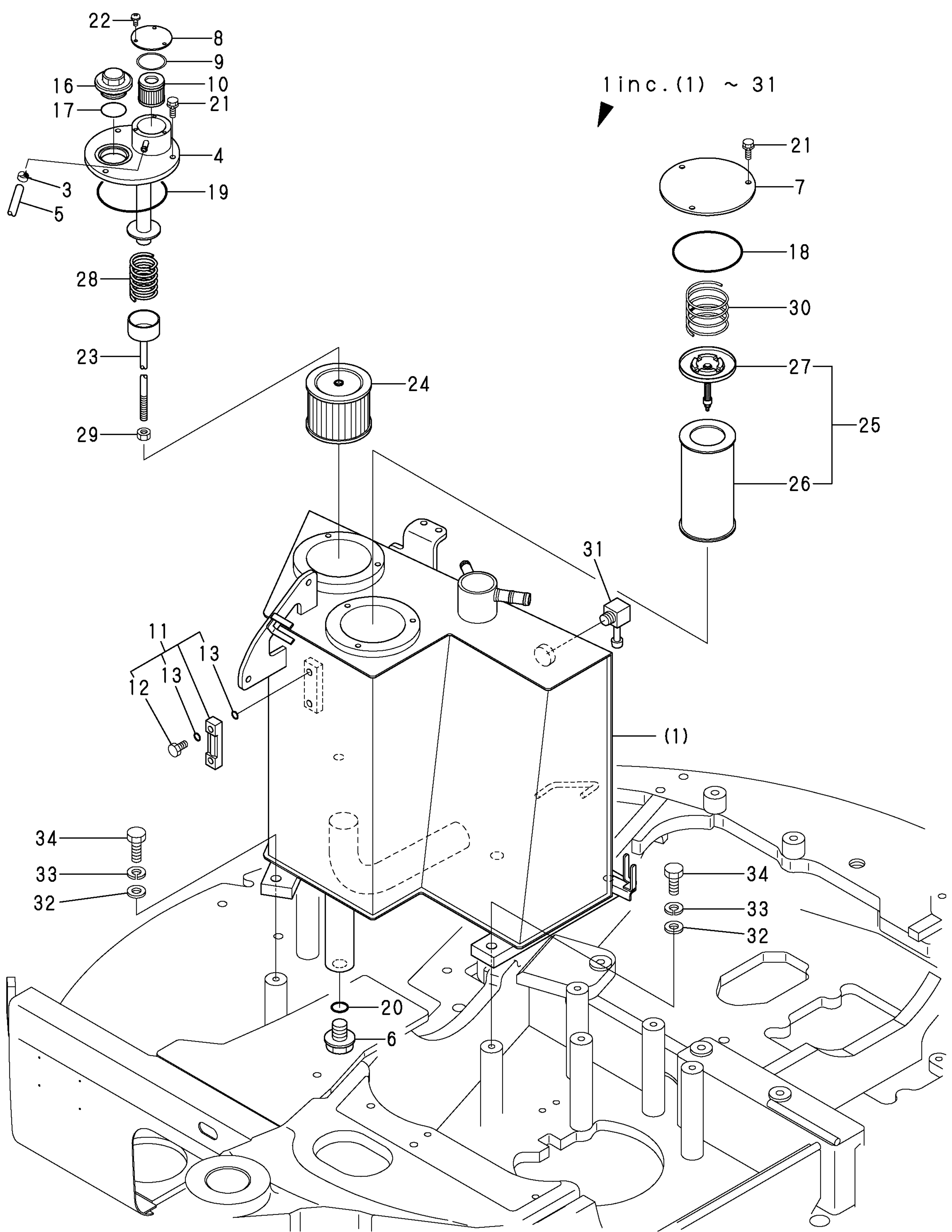
Fig. 42 HYD. OIL TANK
