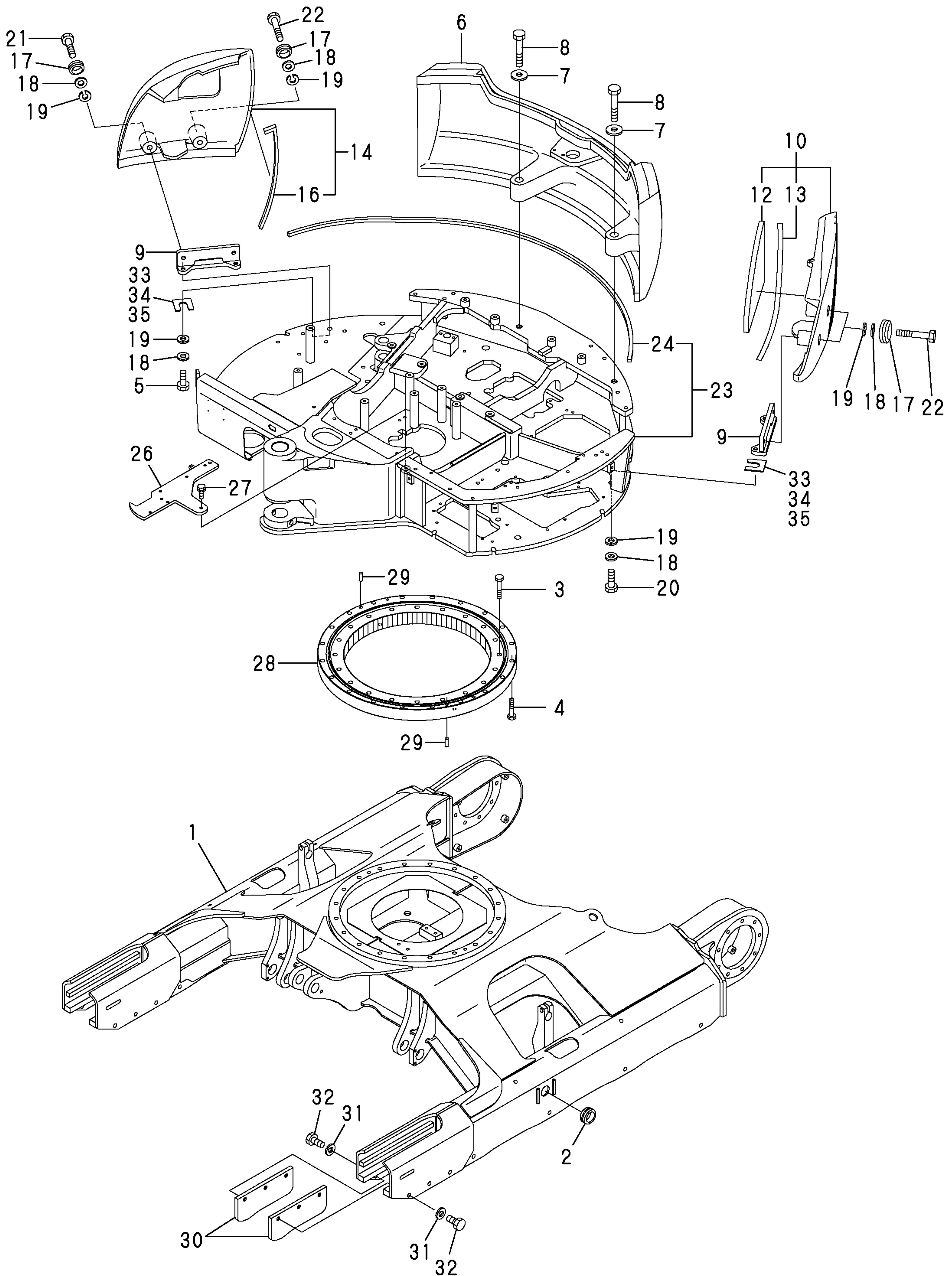
Fig. 20 FRAME & TURNING BEARING
