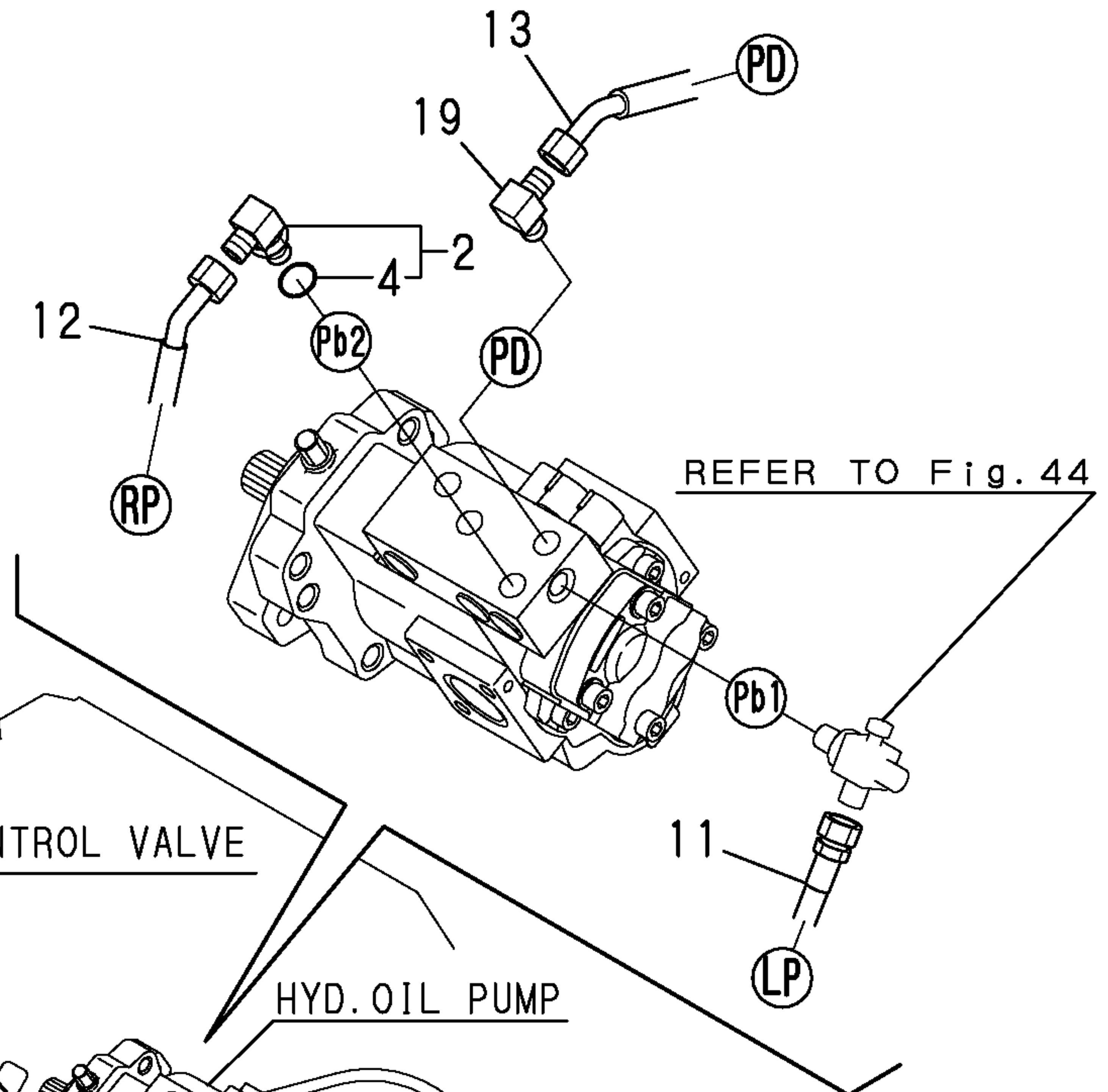
Fig. 50 CON. PIPING (PUMP-VALVE-RETURN)
