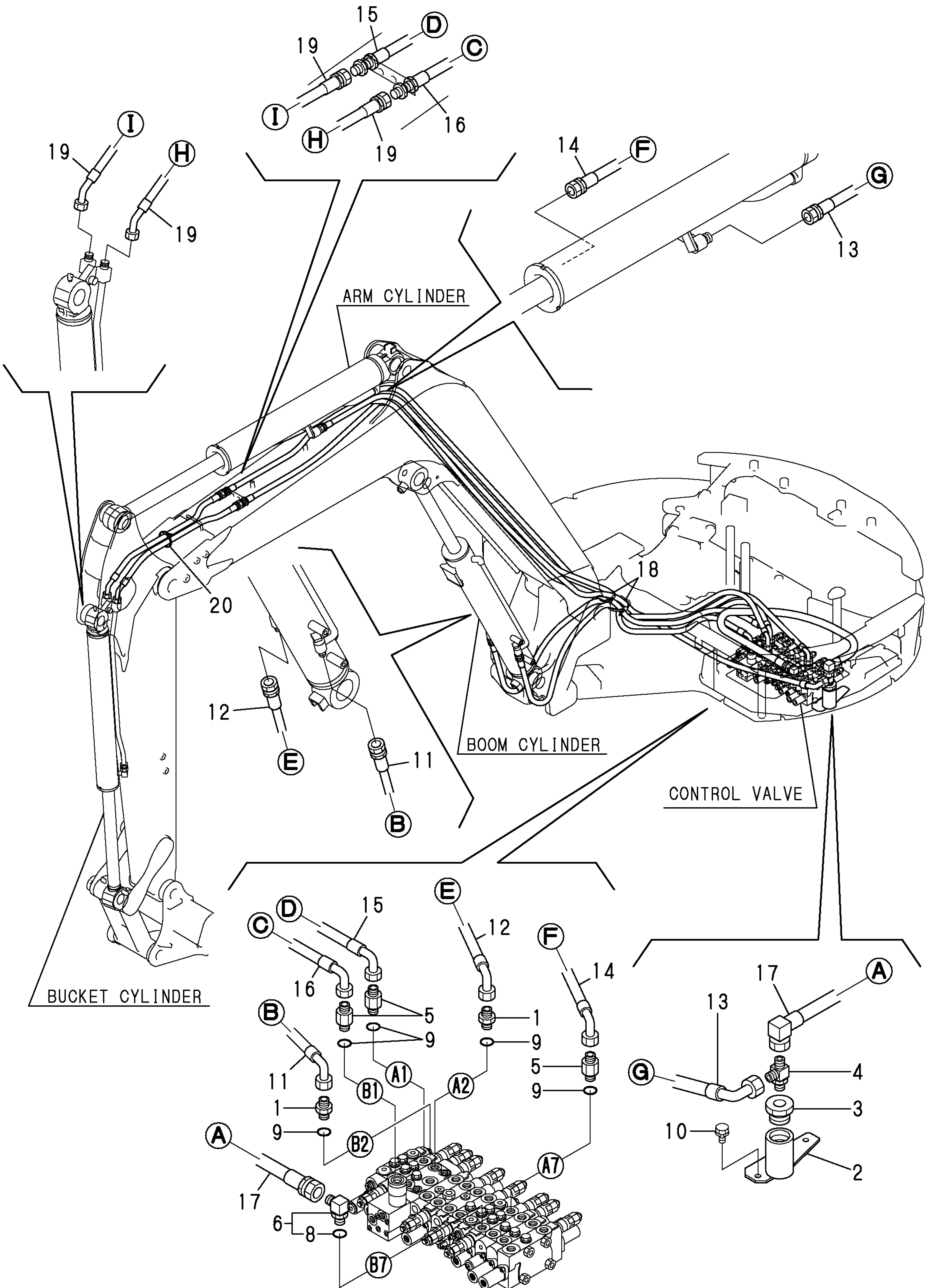
Fig. 48 HYD. OIL PIPING (BOOM)
