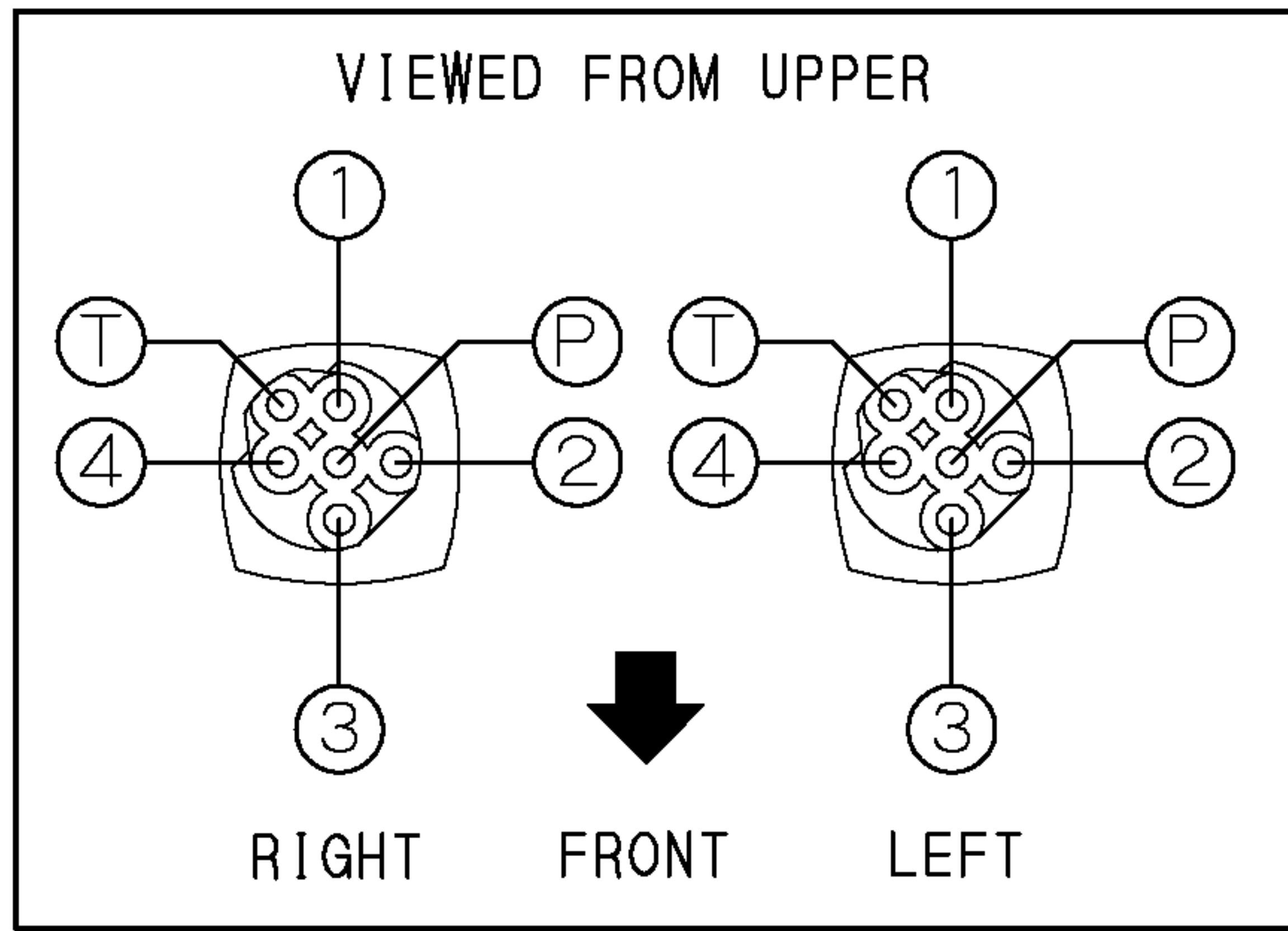
Fig. 51 CON. PIPING (VALVE-CONTROL V.)
