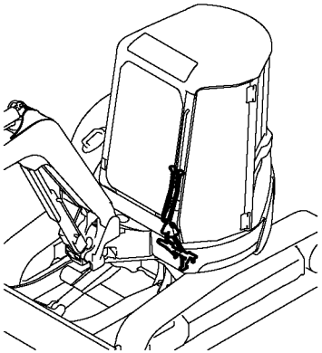
Fig. 16 CONTROL EQUIPMENT (BLADE LEVER)
