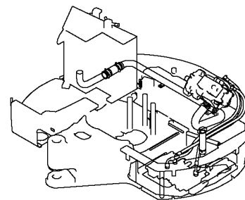
Fig. 44 HYD. OIL PIPING (PUMP-V.-MOTOR)
