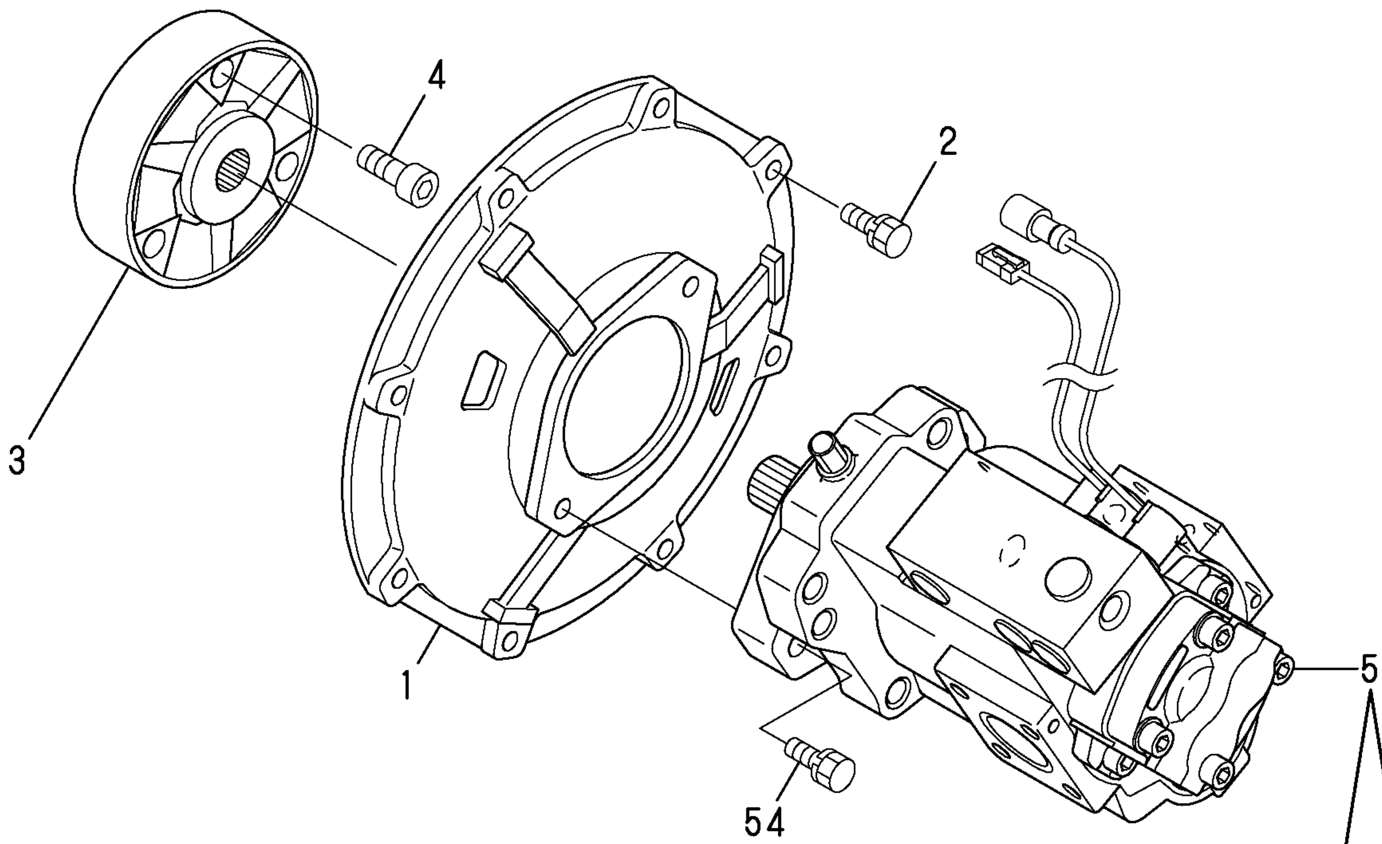
Fig. 27 HYD. OIL PUMP & JOINT
