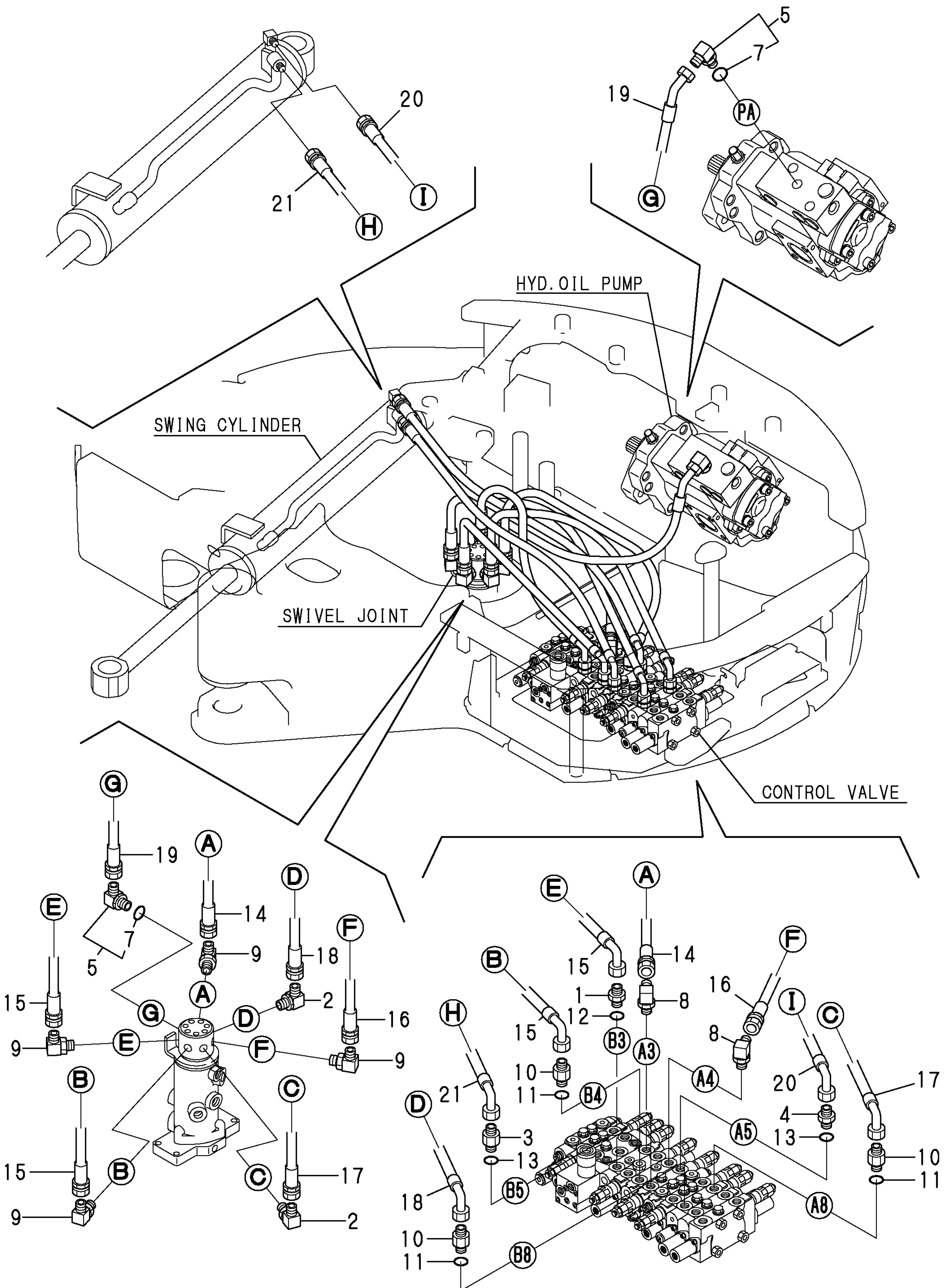
Fig. 45 HYD. OIL PIPING (VALVE-S. -SWING)
