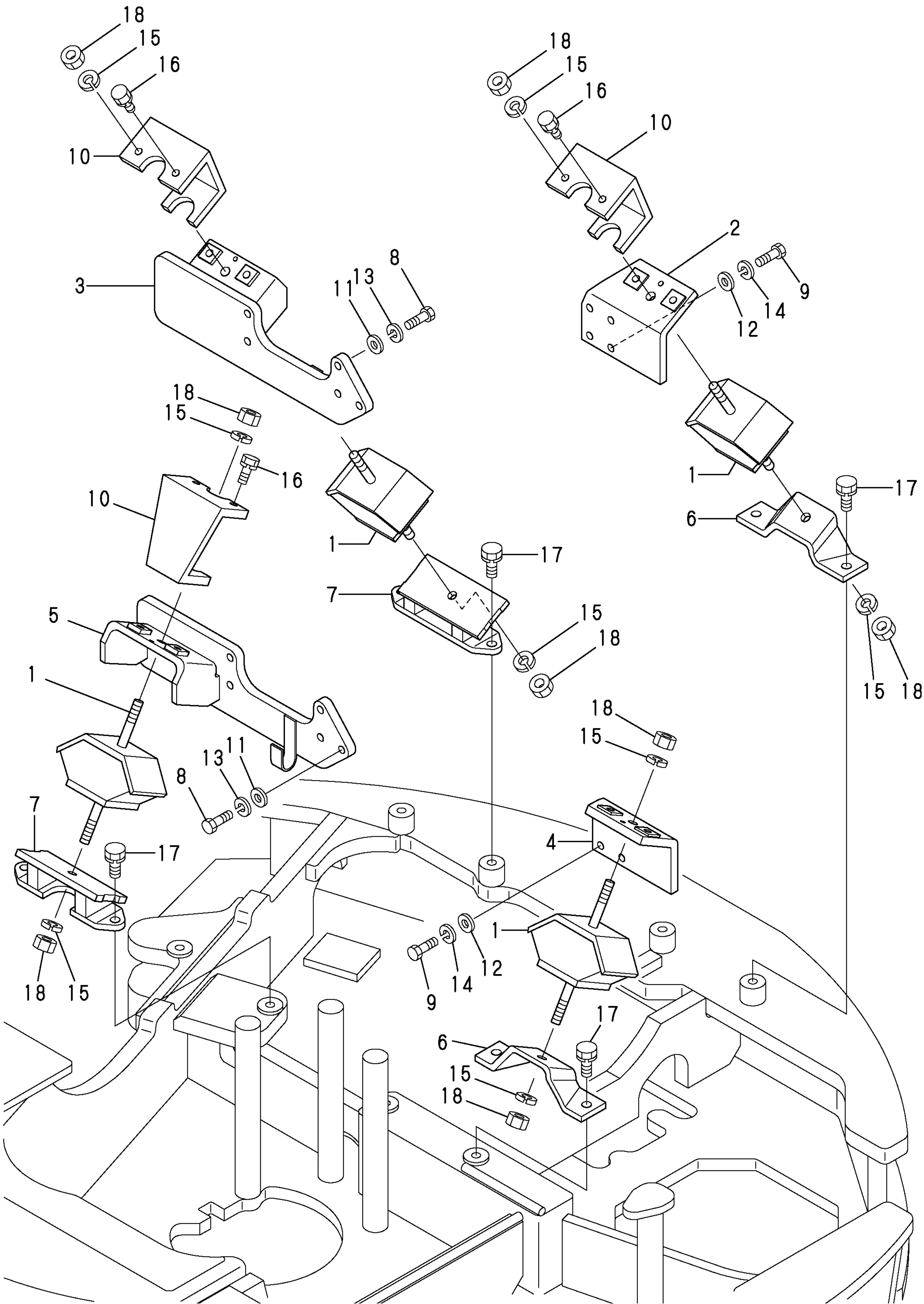
Fig. 4 ENGINE MOUNT
