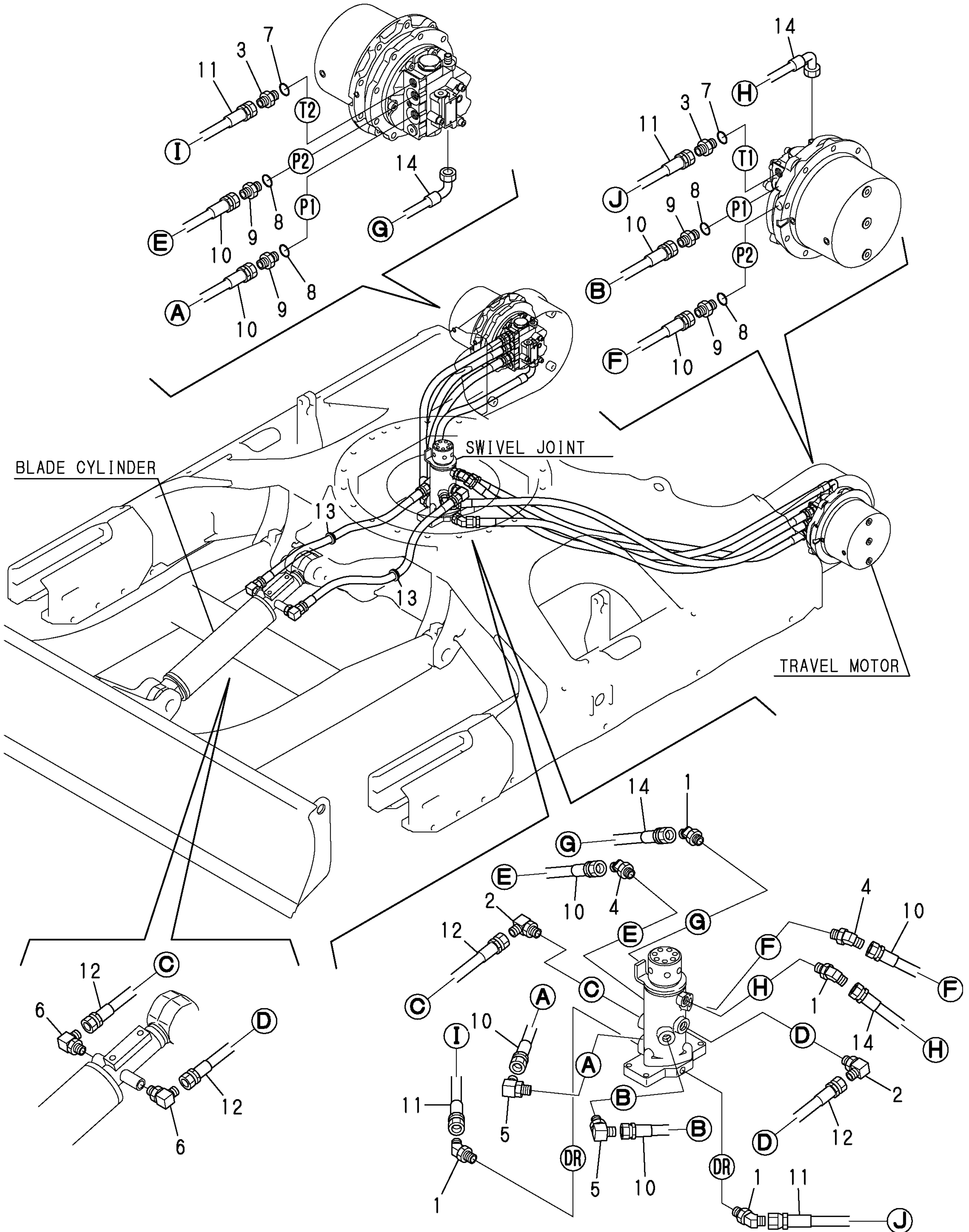
Fig. 47 HYD. OIL PIPING (TRAVEL)
