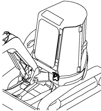
Fig. 19 CONTROL EQUIPMENT (P. T. O. PEDAL)
