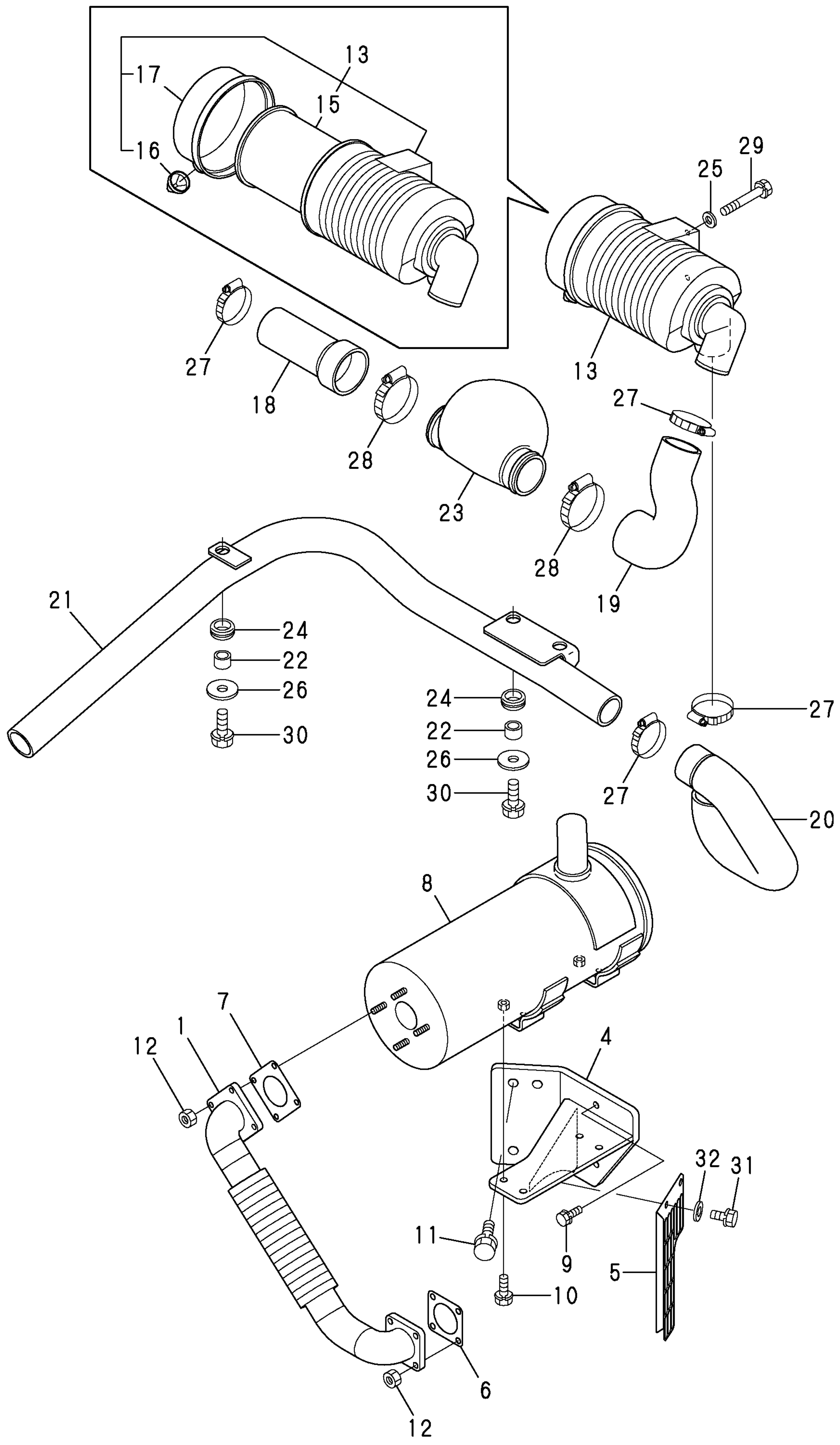
Fig. 2 SILENSER & AIR CLEANER
