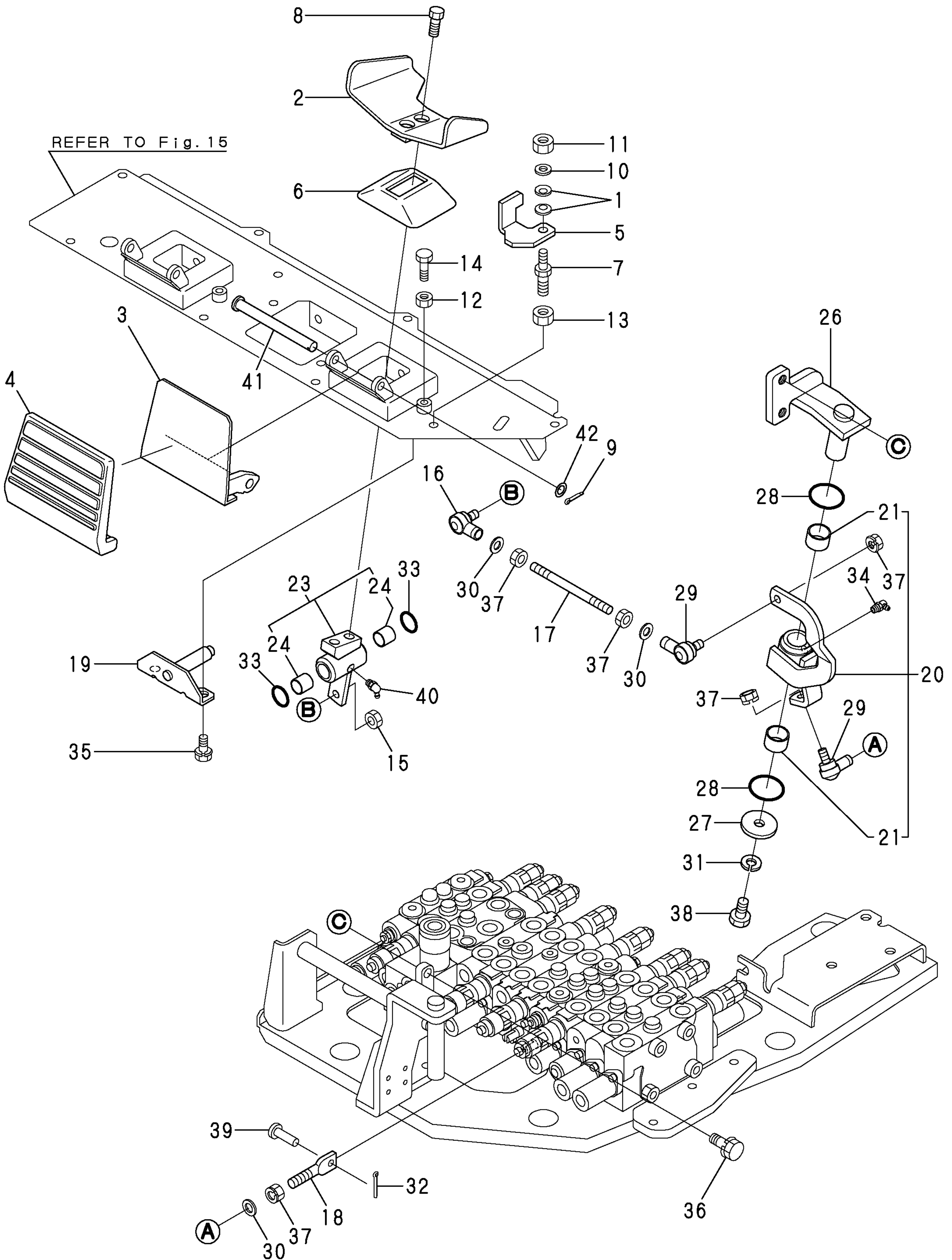
Fig. 19 CONTROL EQUIPMENT (P. T. O. PEDAL)
