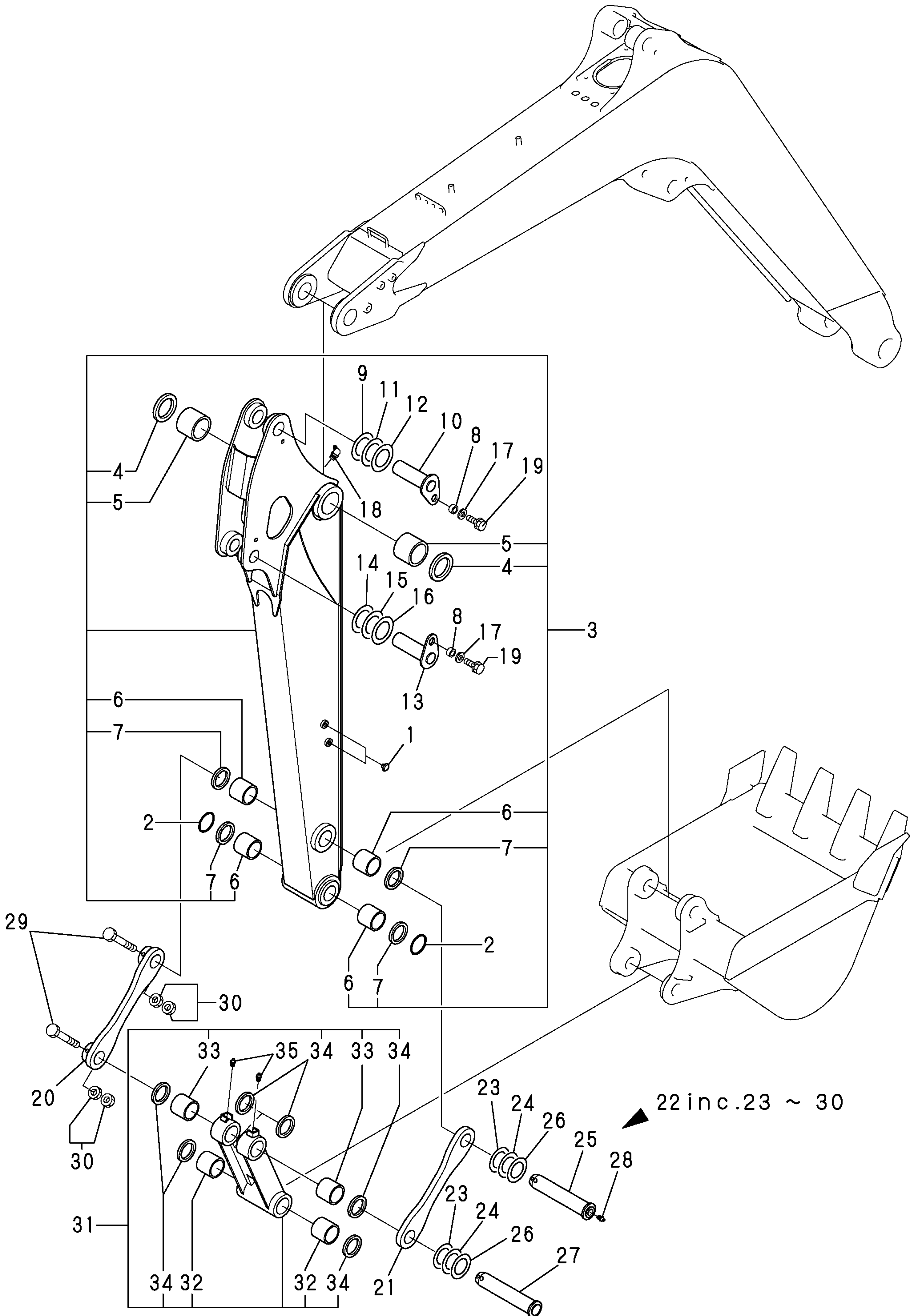
Fig. 54 ARM & BUCKET LINK
