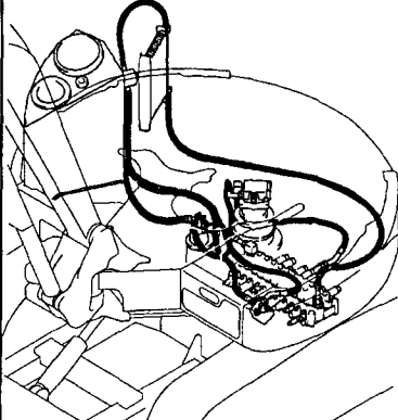
Fig.70 油圧配管 (リターン) (旧形) HYD.OIL PIPING (RETURN) (PREVIOUS)
