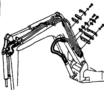
Fig.76 油圧配管 (ブーム) HYD. OIL PIPING (BOOM)
