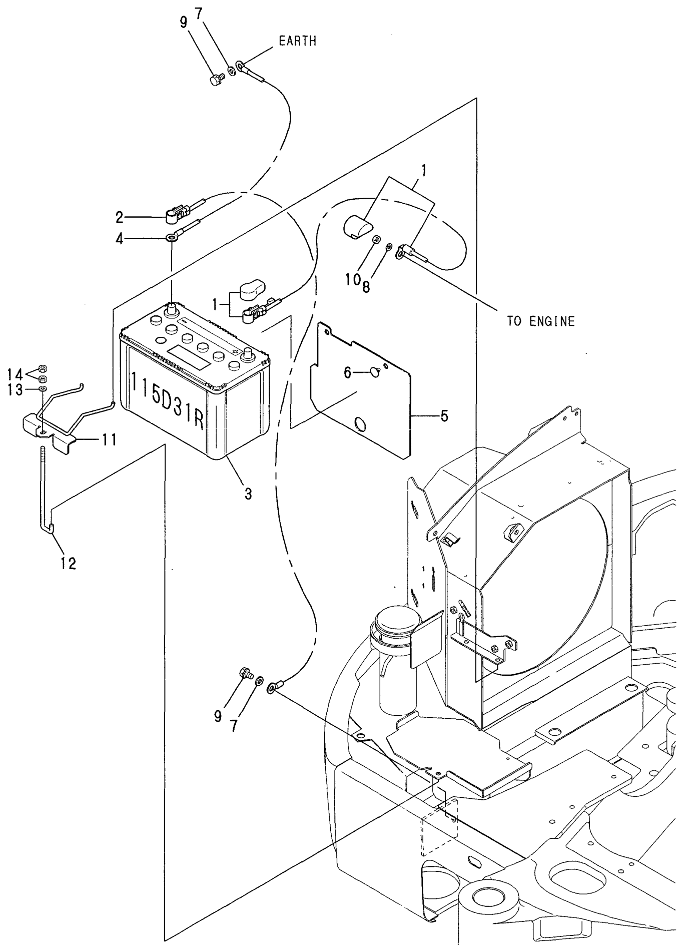
Fig. 8 BATTERY
