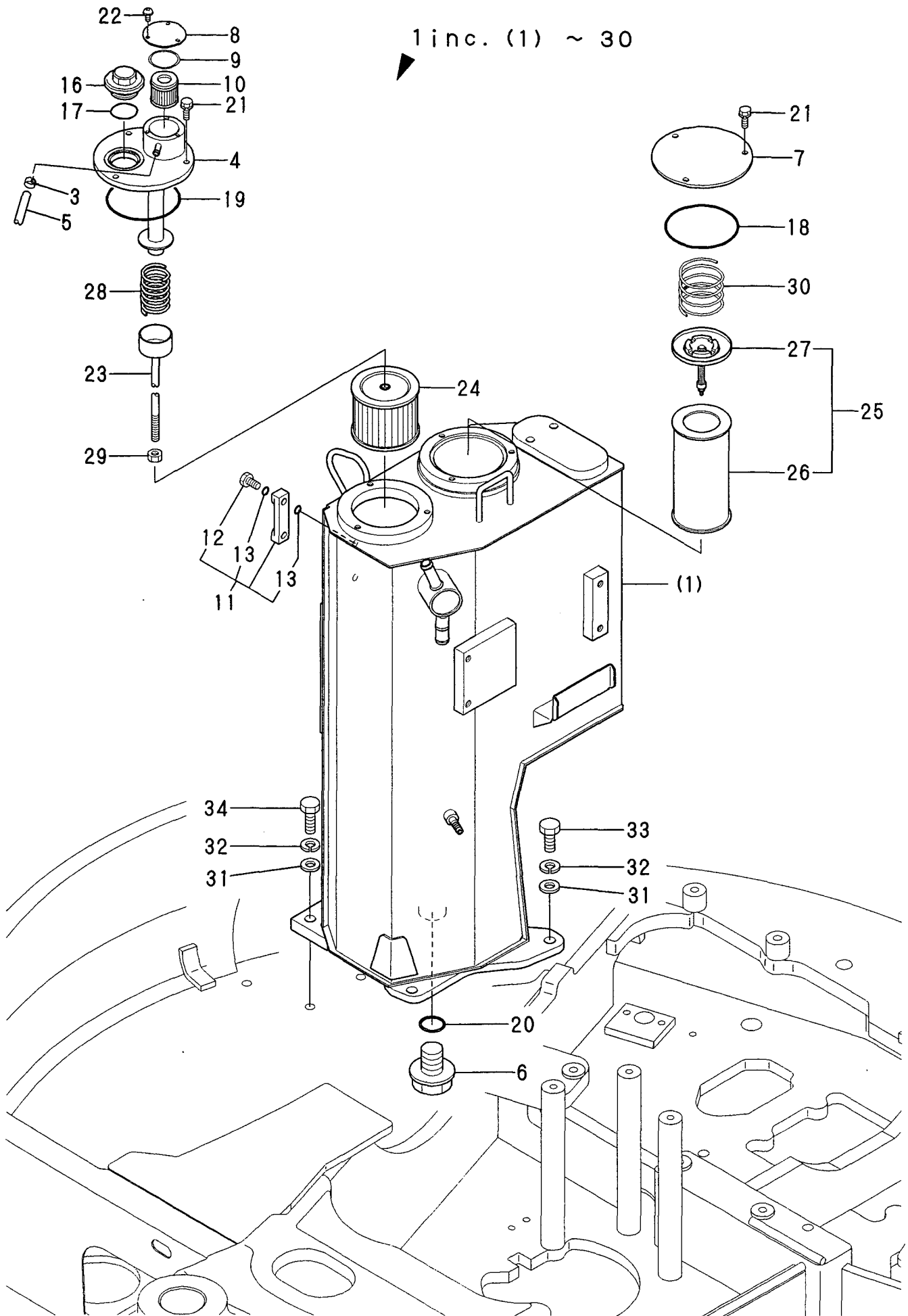
Fig. 43 HYD. OIL TANK
