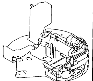
Fig. 44 HYD. OIL PIPING (TANK~PUMP~VALVE)
