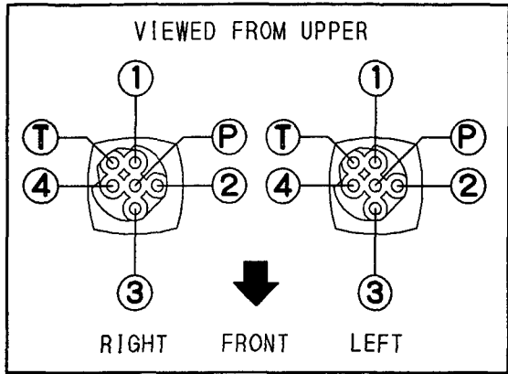
Fig. 52 CONTROL PIPING (REMO.-CON. V. ~CONTROL V.)
