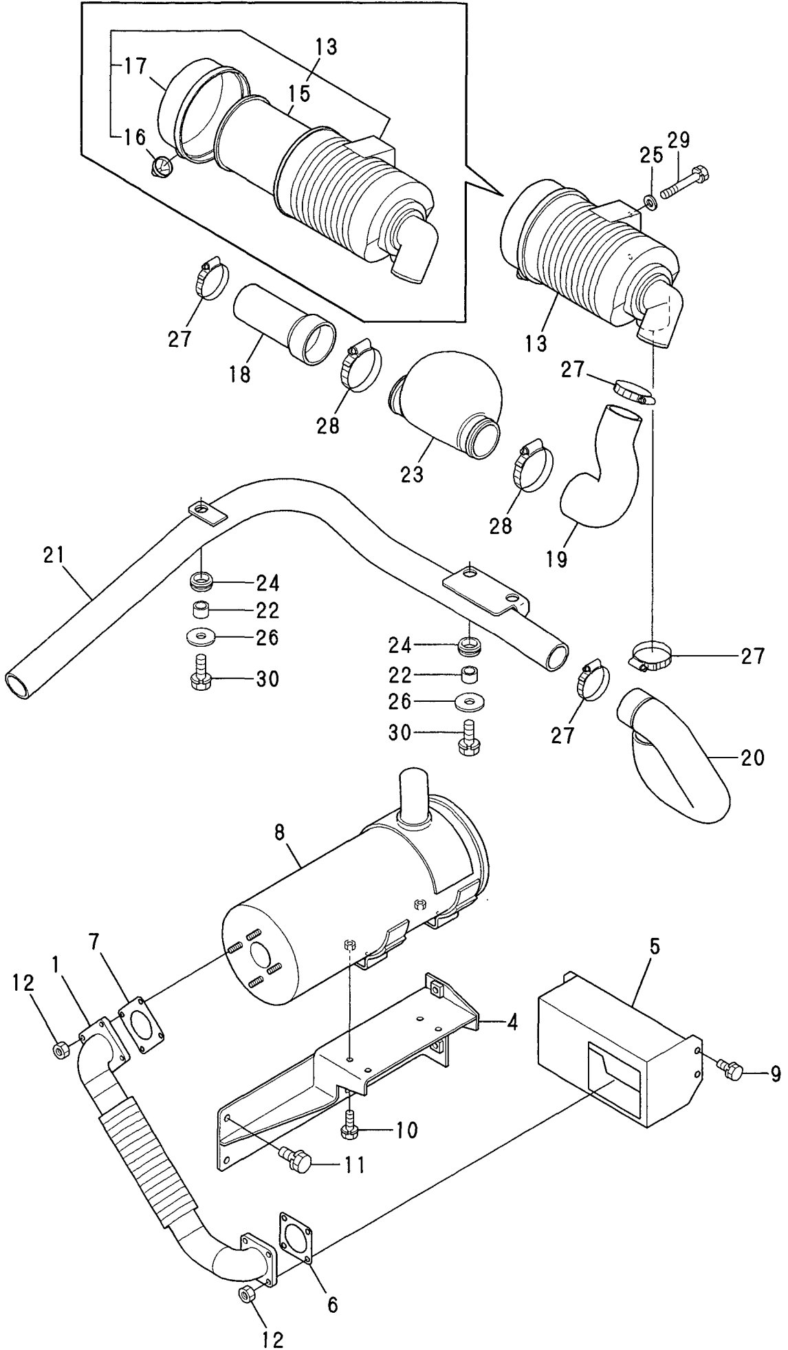
Fig. 3 SILENSER & AIR CLEANER
