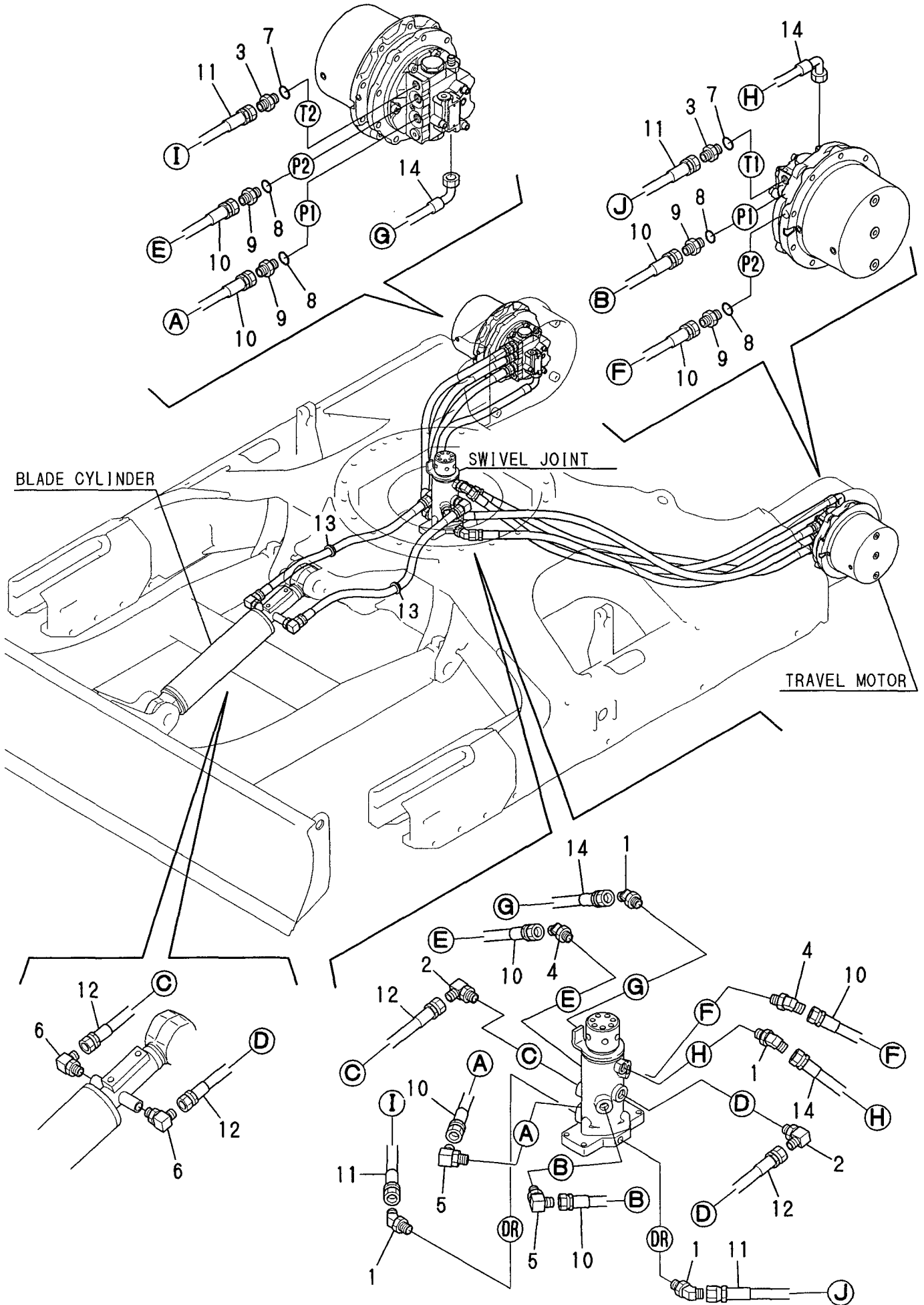
Fig. 48 HYD. OIL PIPING (TRAVEL)
