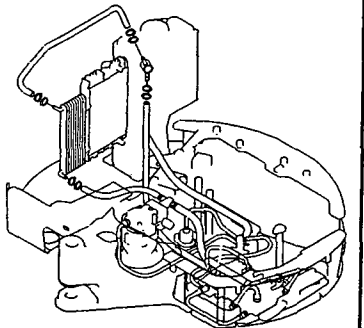
Fig. 47 HYD. OIL PIPING (RETURN)
