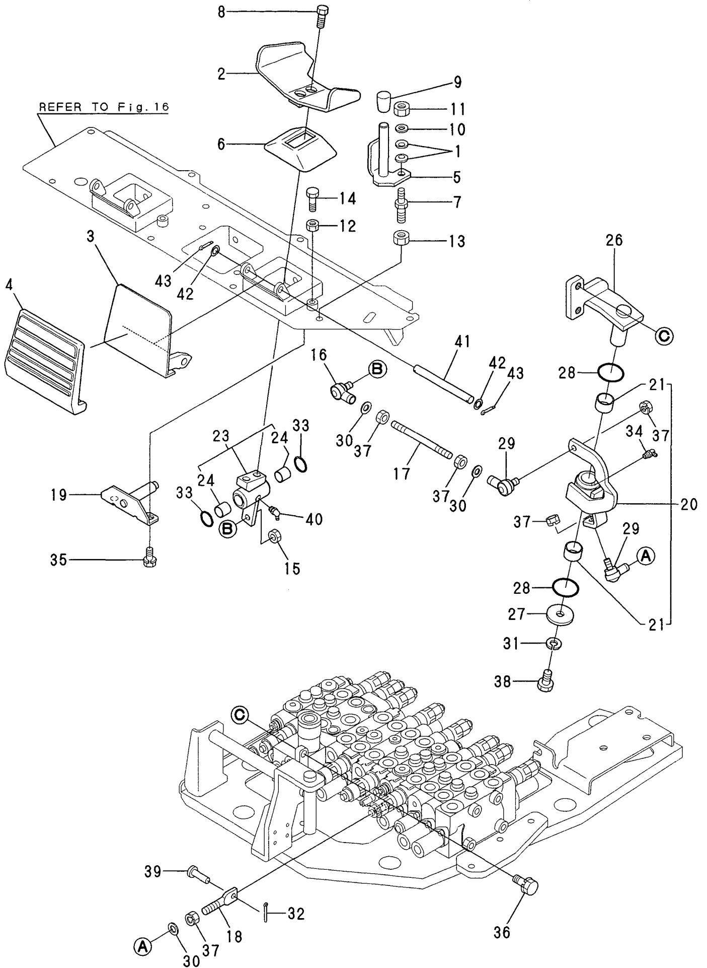
Fig. 20 CONTROL EQUIPMENT (P. T. O. PEDAL)
