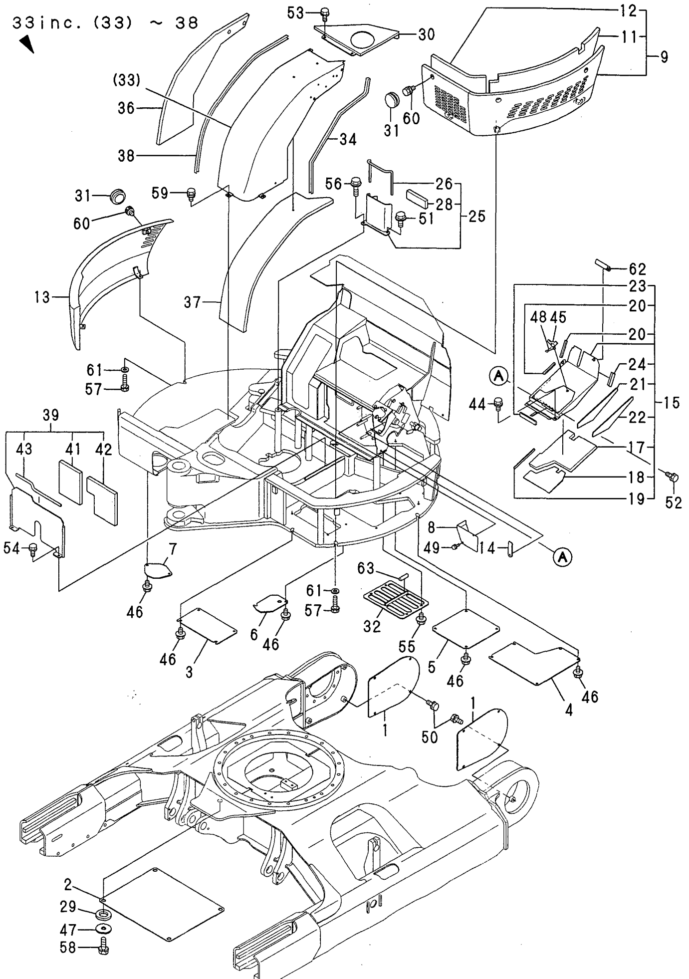
Fig. 22 COVER (FRAME)
