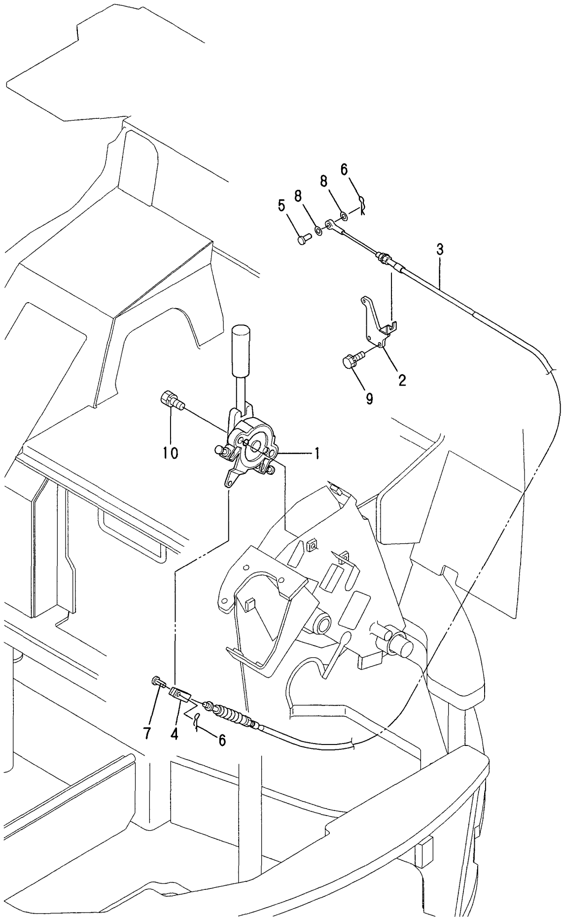
Fig. 4 ACCELERATOR
