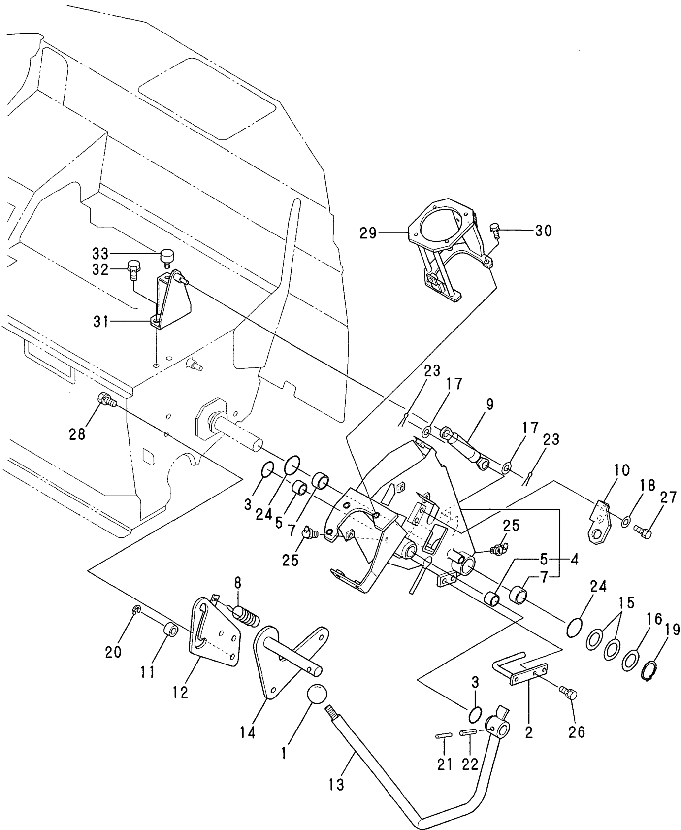
Fig. 15 CONTROL EQUIPMENT (LOCK LEVER & STAND) LEFT
