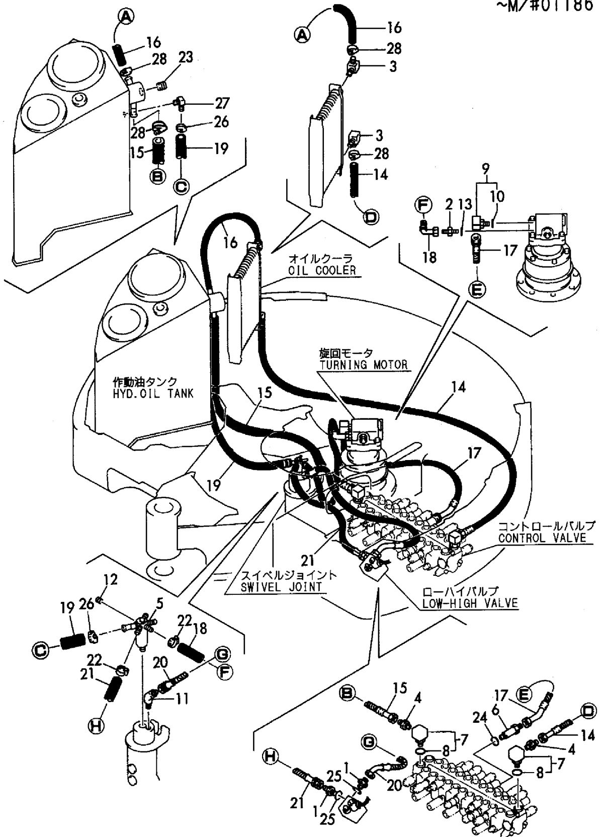
Fig. 80 油圧配管 (リターン) (旧形) HYD. OIL PIPING (RETURN) (PREVIOUS)
