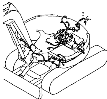
Fig.19 電装品 (キャビン) ELECTRIC PART (CABIN)
