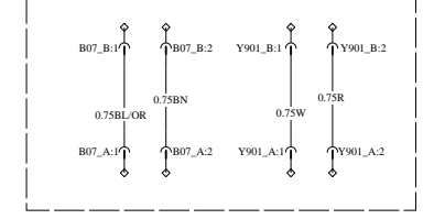
Cable extension for Y901 and B07 (location: Wiring Diagram NA)
