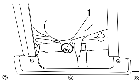
1. Engine oil drain bolt (crankcase)
