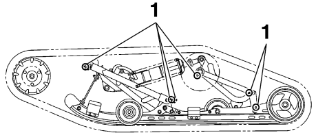
1. Lubrication point
