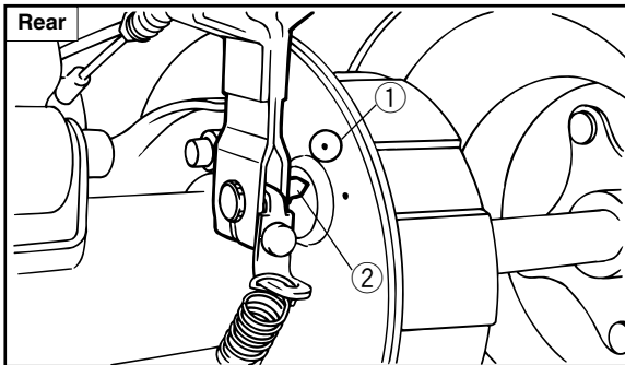
1. Wear limit mark
