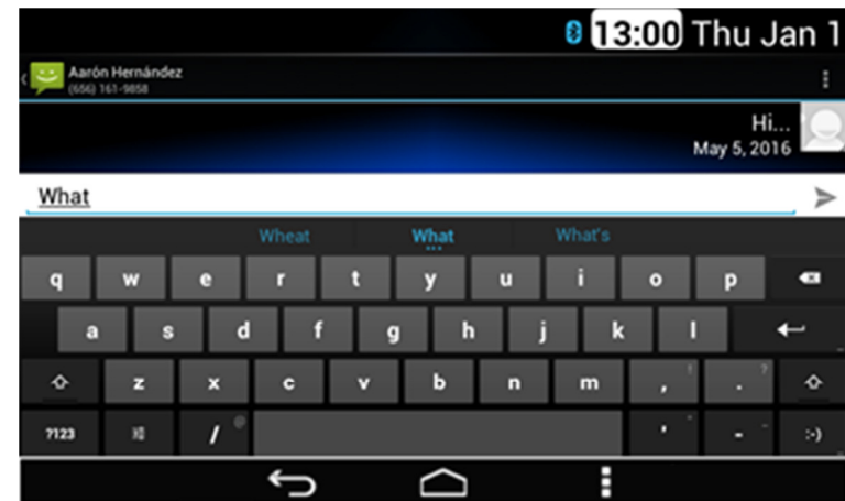
Figure 63: Message editor
