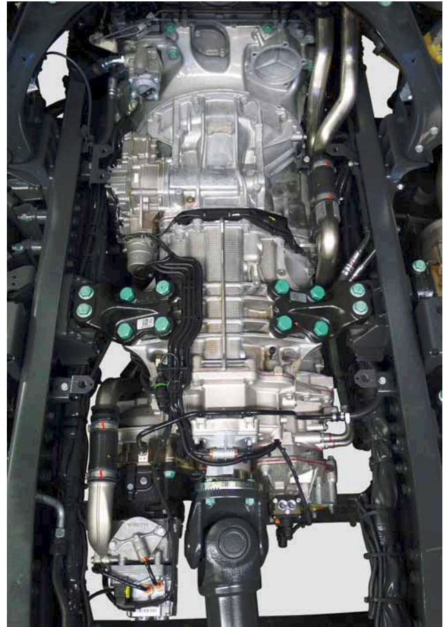
Transmission G 330-12 (G1F)
