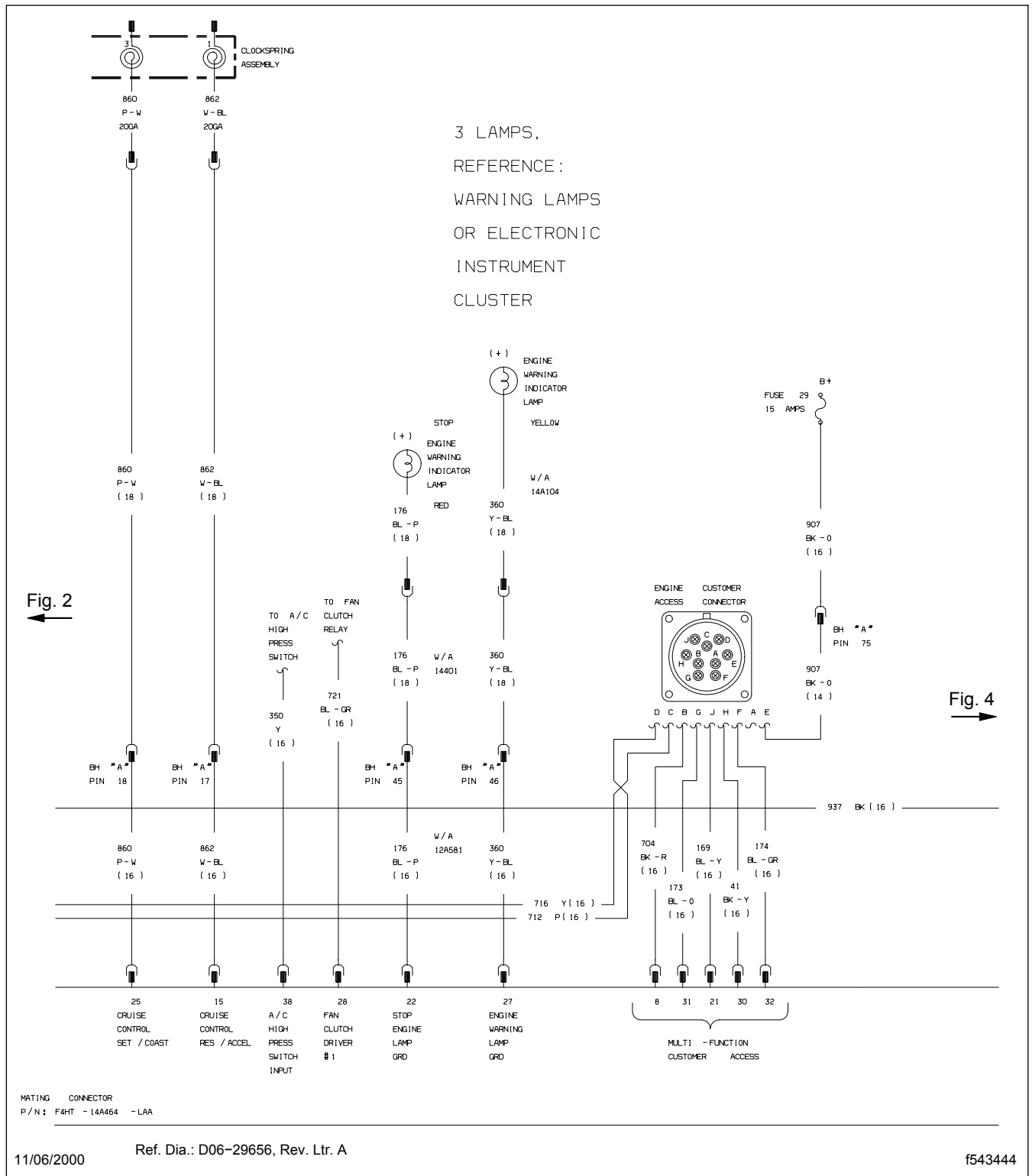
Fig. 3, Caterpillar C10, C12 and 3406 Engine Controls Wiring (partial view)
