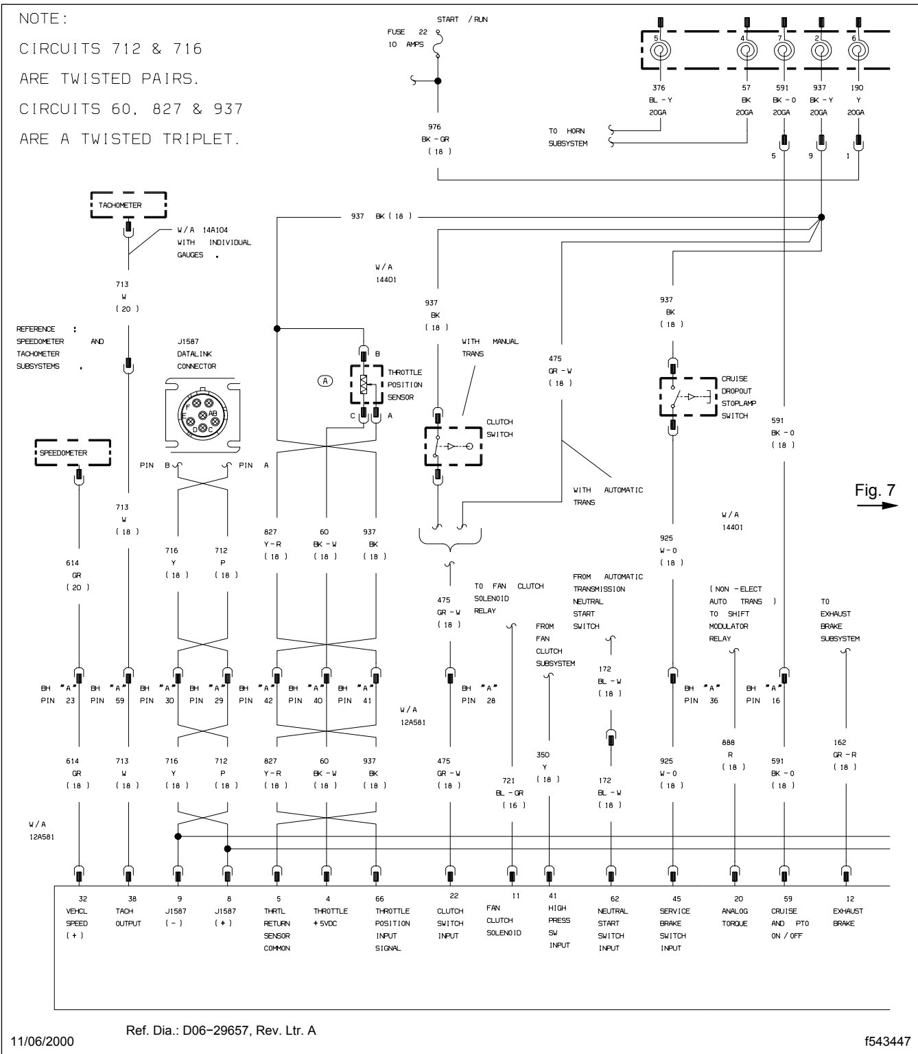
Fig. 6, Caterpillar 3126 Engine Controls Wiring (partial view)
