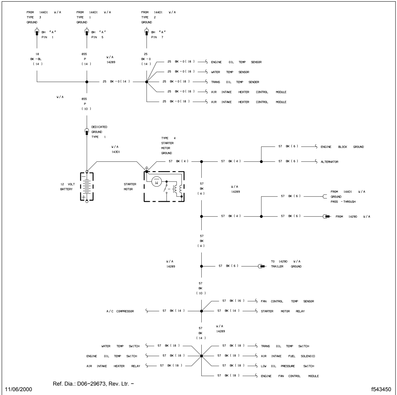
Fig. 9, Caterpillar 3306 Engine Ground Summary (full view)
