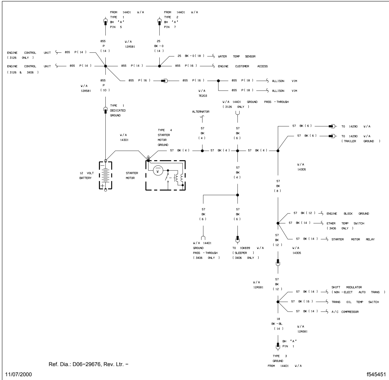
Fig. 10, Caterpillar 3126 and 3406 Engine Ground Summary (full view)
