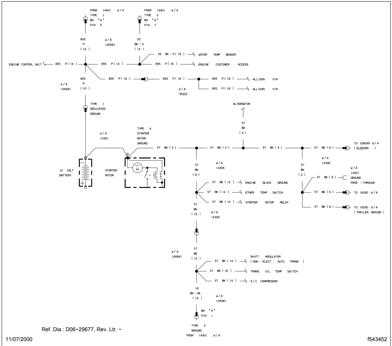
Fig. 11, Caterpillar C10 and C12 Engine Ground Summary (full view)
