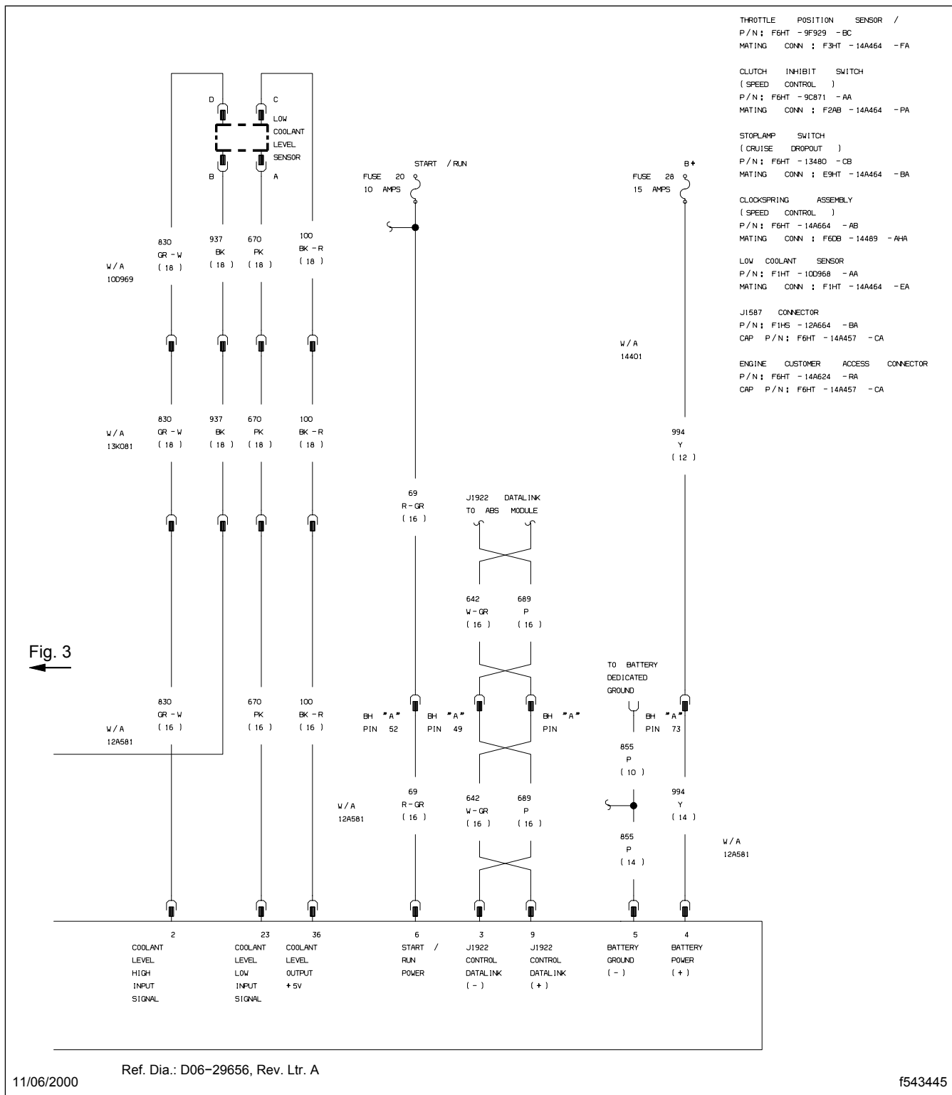
Fig. 4, Caterpillar C10, C12 and 3406 Engine Controls Wiring (partial view)
