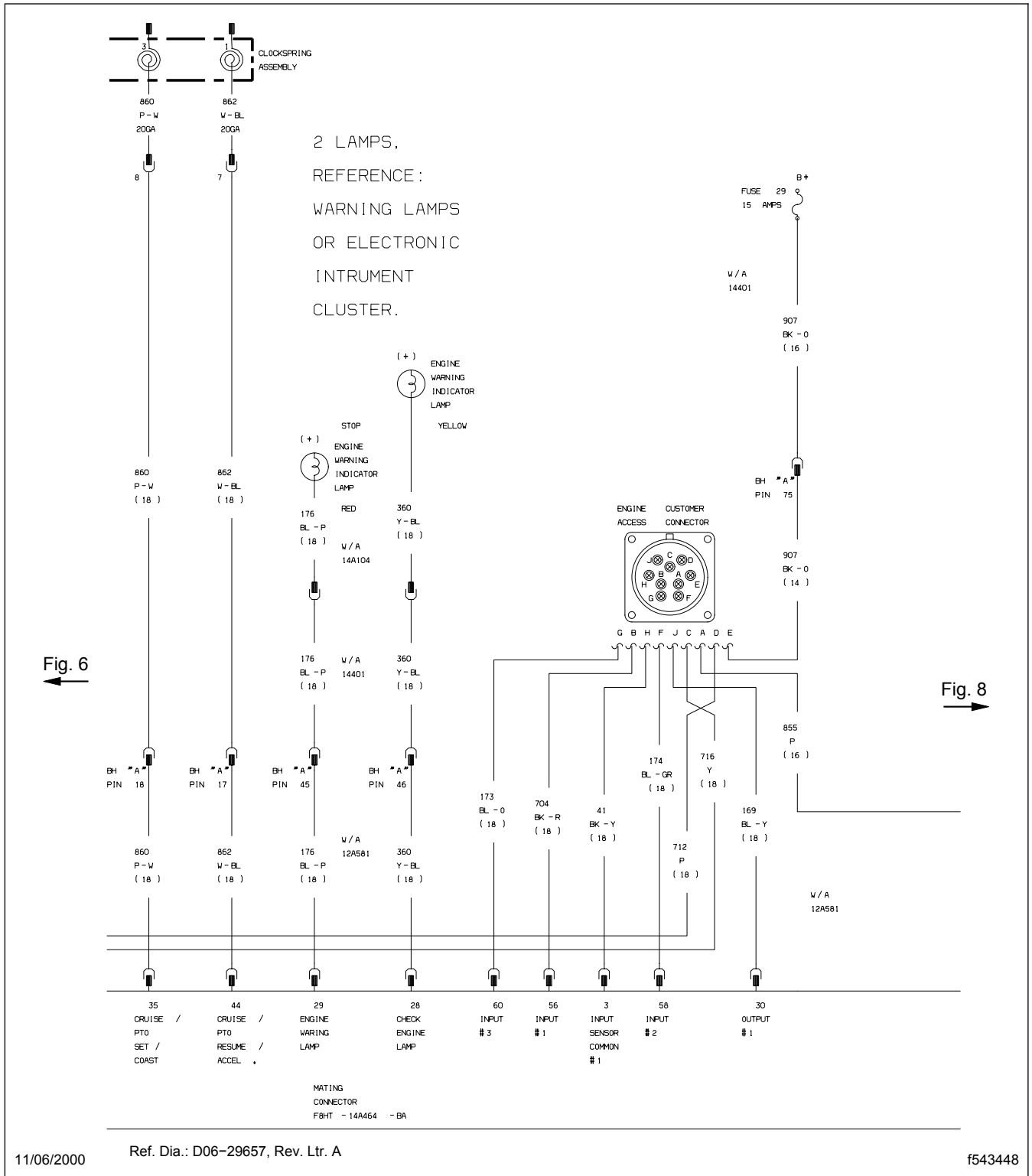
Fig. 7, Caterpillar 3126 Engine Controls Wiring (partial view)
