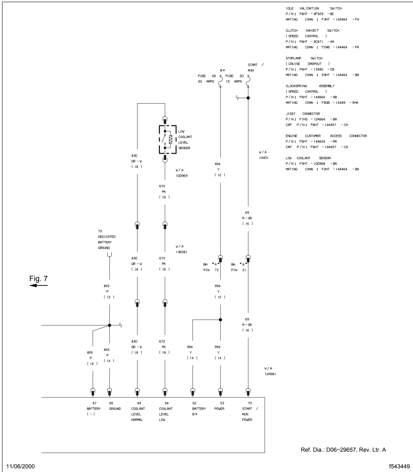
Fig. 8, Caterpillar 3126 Engine Controls Wiring (partial view)
