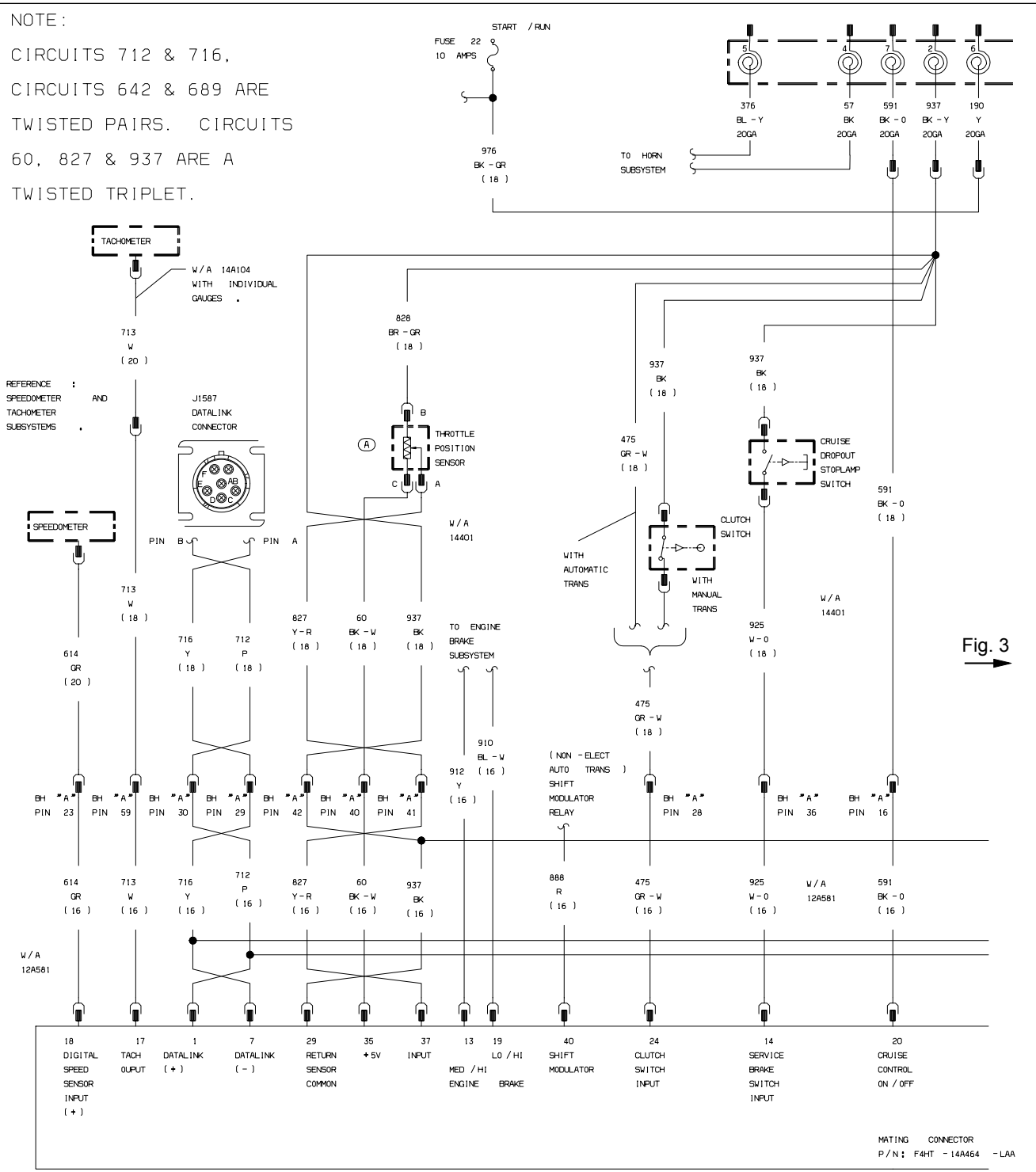
Fig. 2, Caterpillar C10, C12 and 3406 Engine Controls Wiring (partial view)
