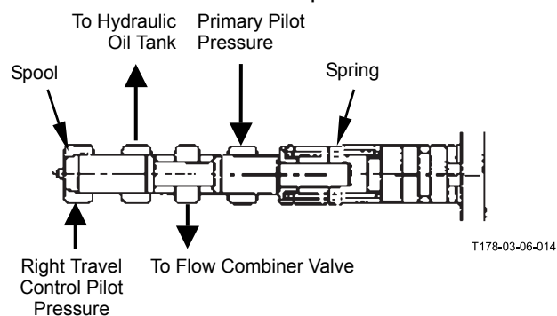
Swing Parking Brake Release Spool:
