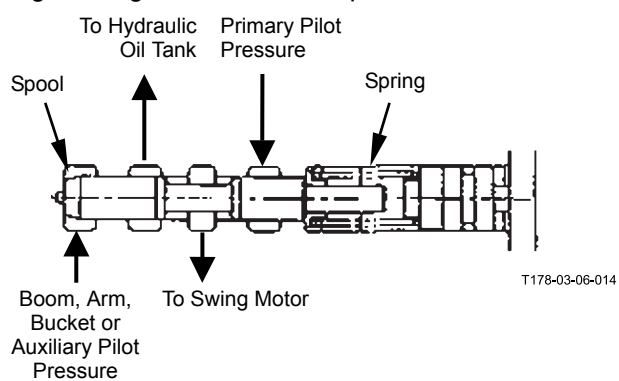
Arm 1 Flow Rate Control Valve Control Spool:
