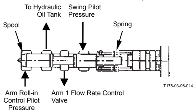
Arm 1 Flow Rate Control Valve Control Spool:
